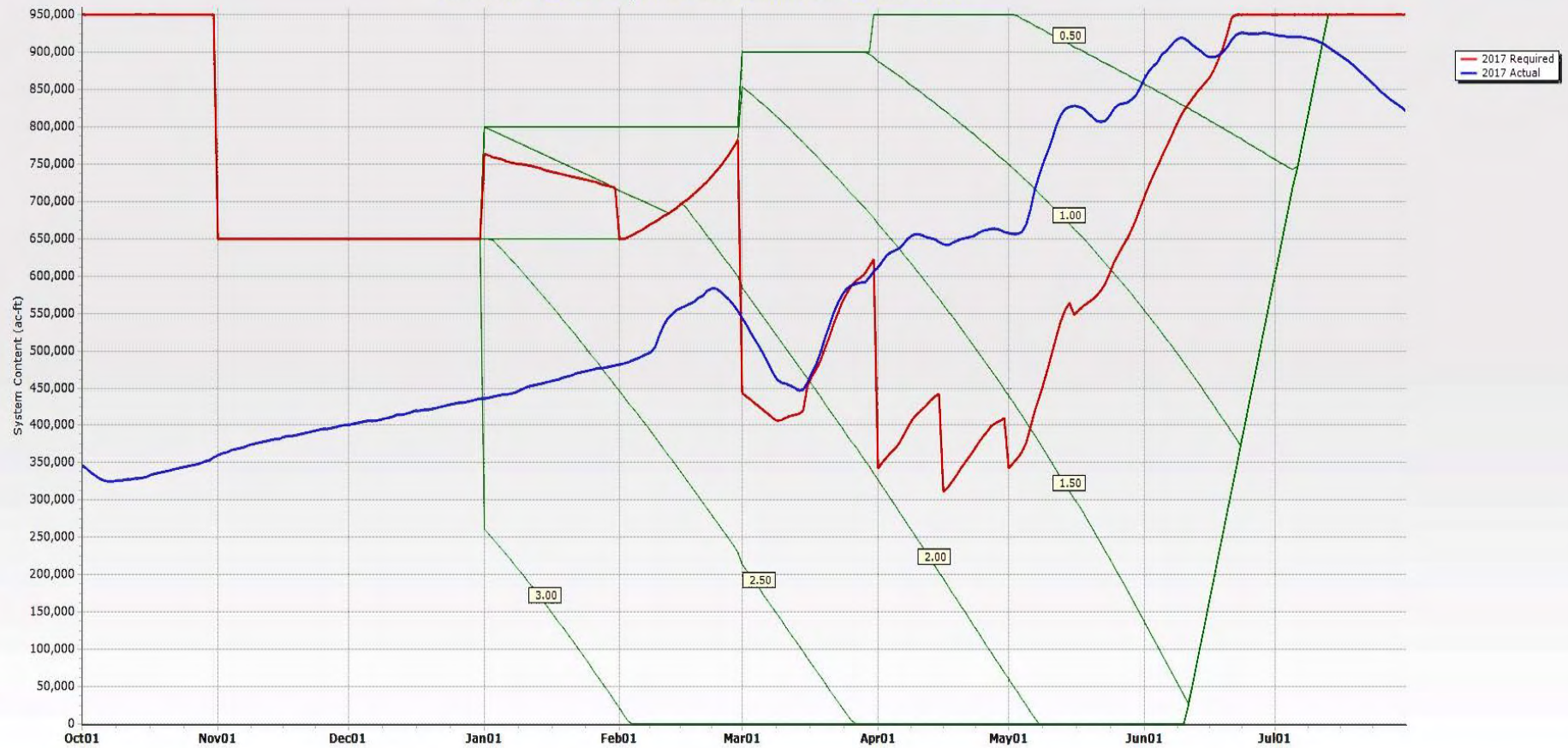
Boise River Reservoir System Flood Control Rule Curves - 2017
