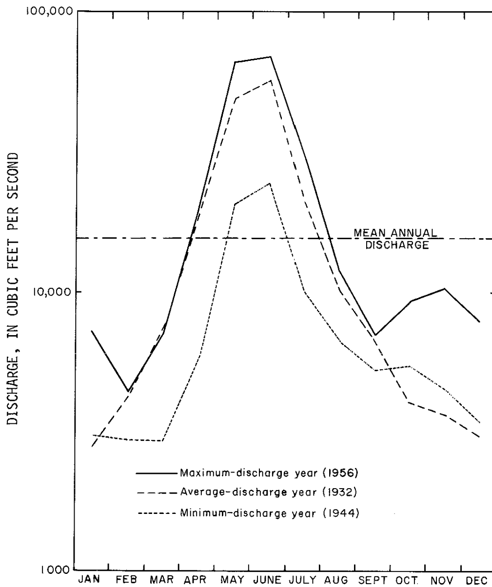
FIGURE 6.--Mean monthly discharge of Kootenai River near Copeland (12318500) for selected years.
