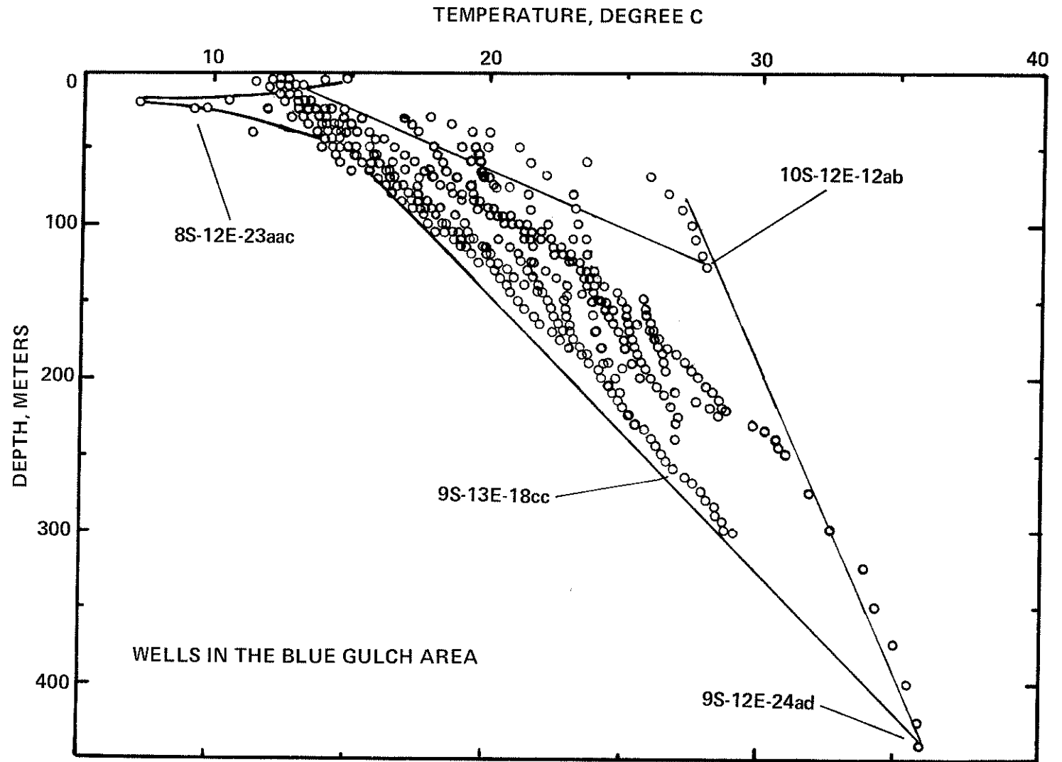
FIGURE 19. Temperature-depth plots of the measured wells in the Blue Gulch area.
