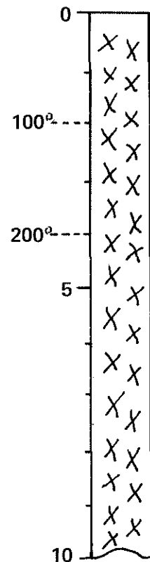
FIGURE 13. One-dimensional geologic models of the western Snake River Plain. The interpretive models are based on data and cross sections of Hill and Pakiser (1966), Malde and Powers (1962), Taubeneck (1971), Mabey (1976), and Bowen and Blackwell (1975). The 100 and 200°C temperatures are calculated values using the heat flow values and the mean annual surface temperatures shown and the values of thermal conductivity, density, and specific heat shown in table 5.
