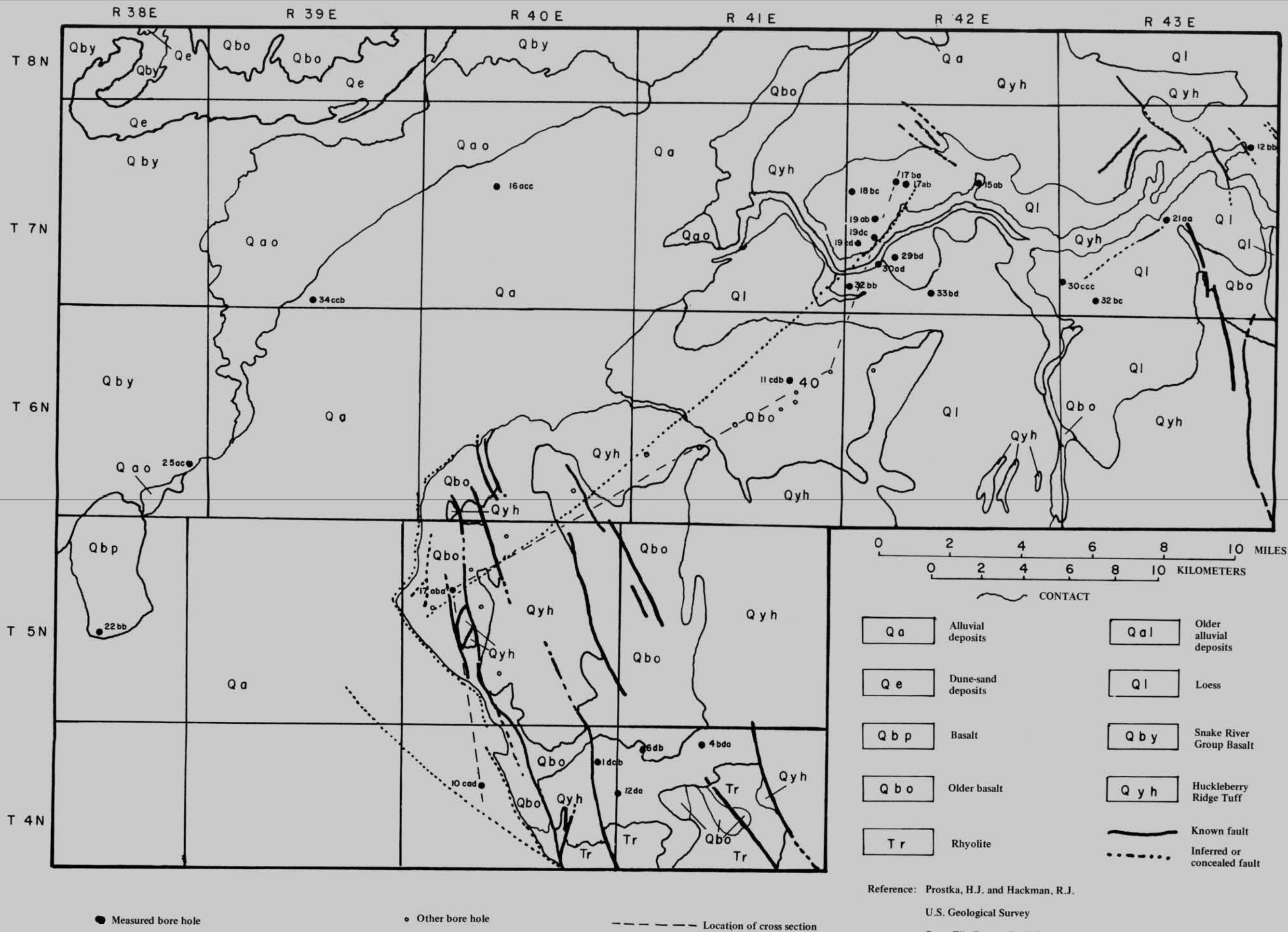
PLATE 3. Geologic map of Rexburg-St. Anthony area.
