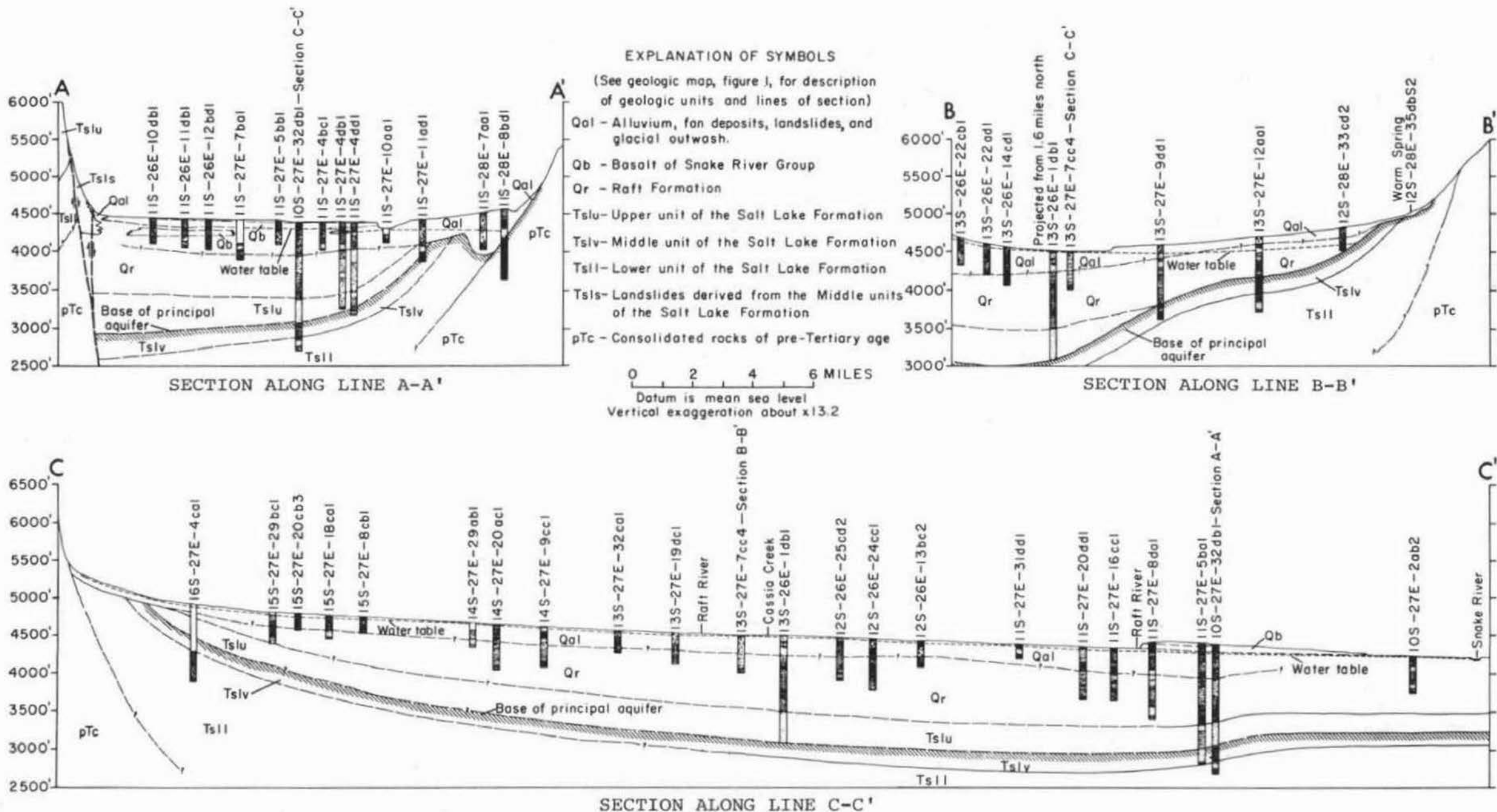
FIGURE 7.--Geologic sections Raft River valley, Idaho.
