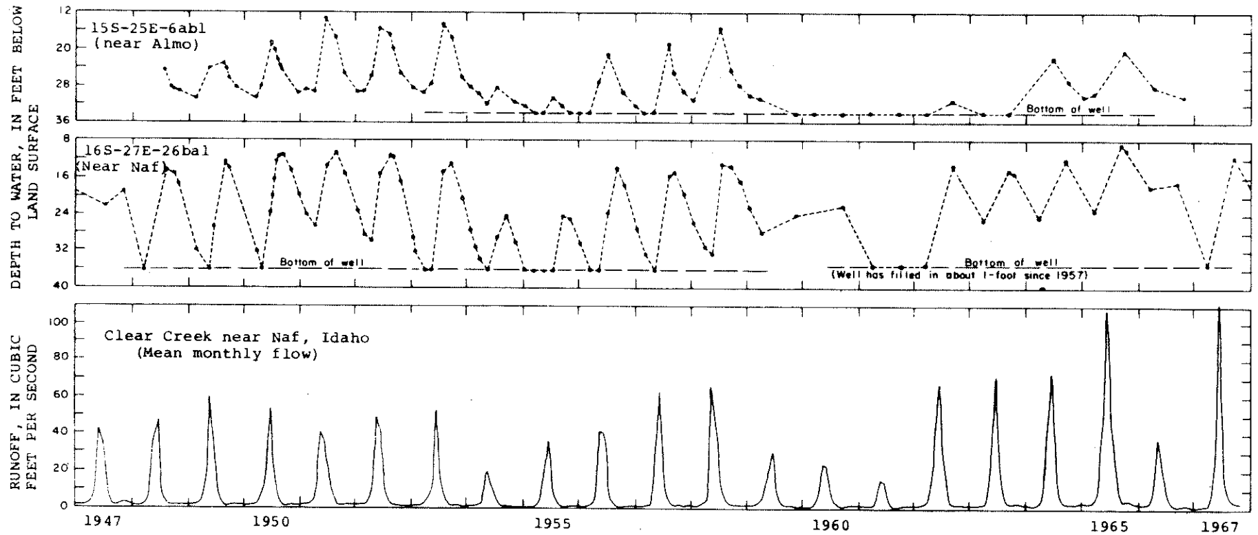
FIGURE 15.— Hydrographs of selected wells in southern part of Raft River basin, and runoff of Clear Creek near Naf.
