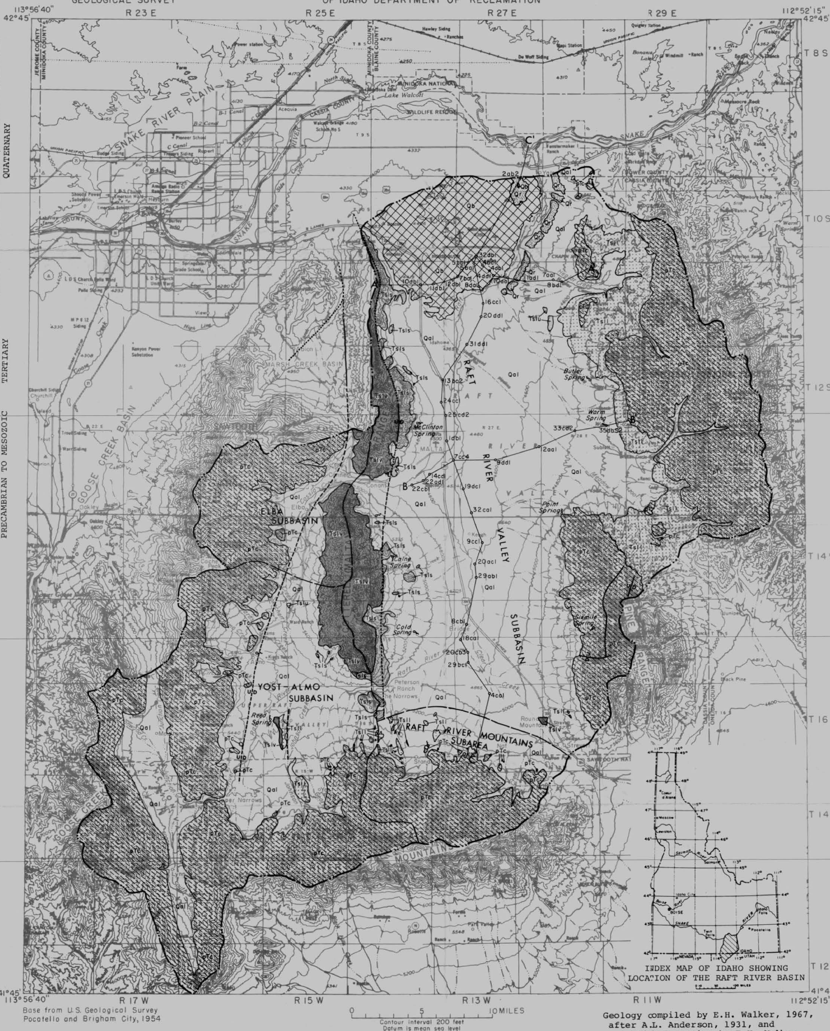
FIGURE 1.--Map of the Raft River basin, Idaho and Utah, showing geology, subbasins and subareas, physiographic features, and lines of geologic sections
