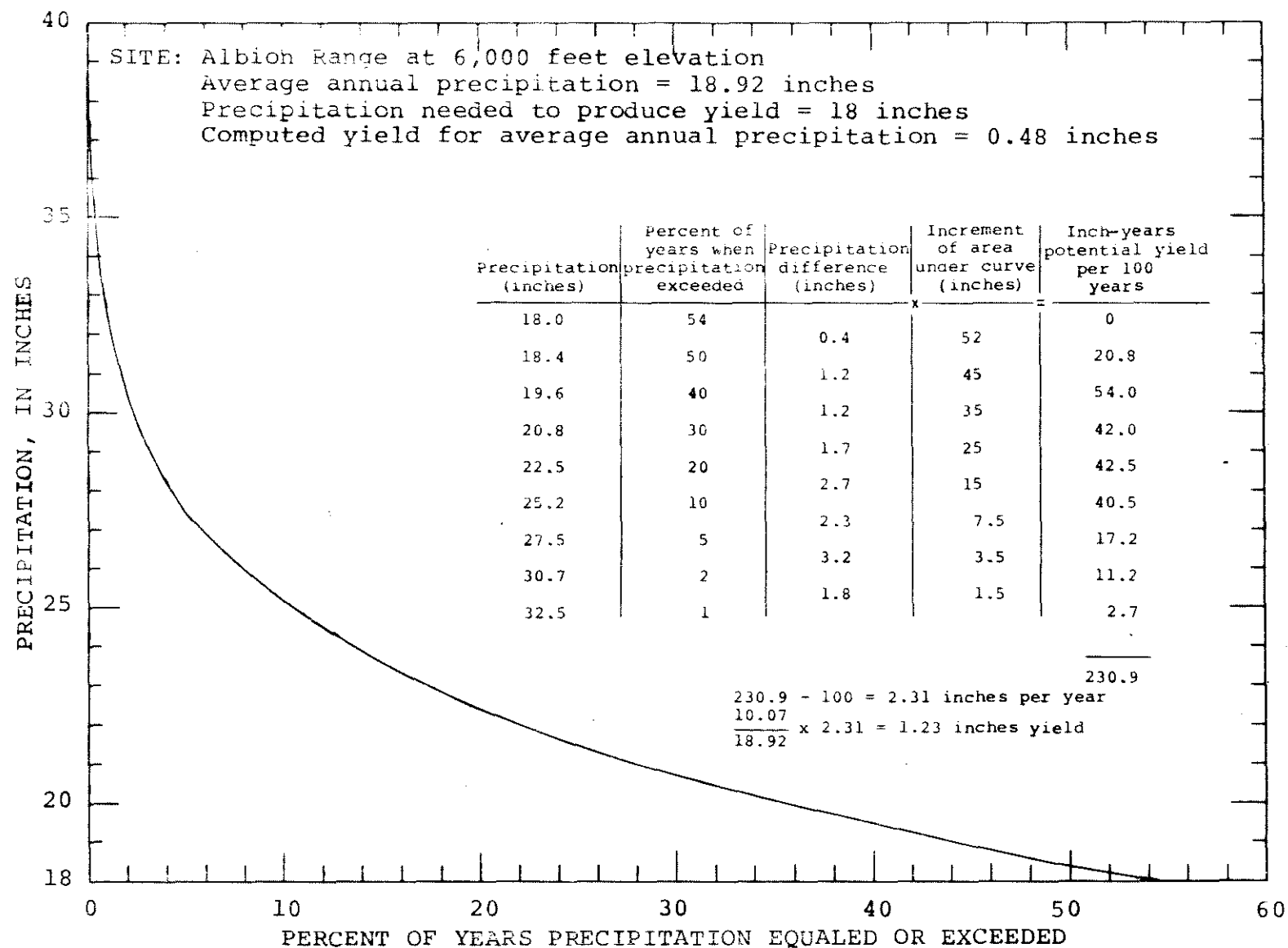
FIGURE 12.-- Annual precipitation in excess of average at a selected site, and computed long-term annual water yield.
