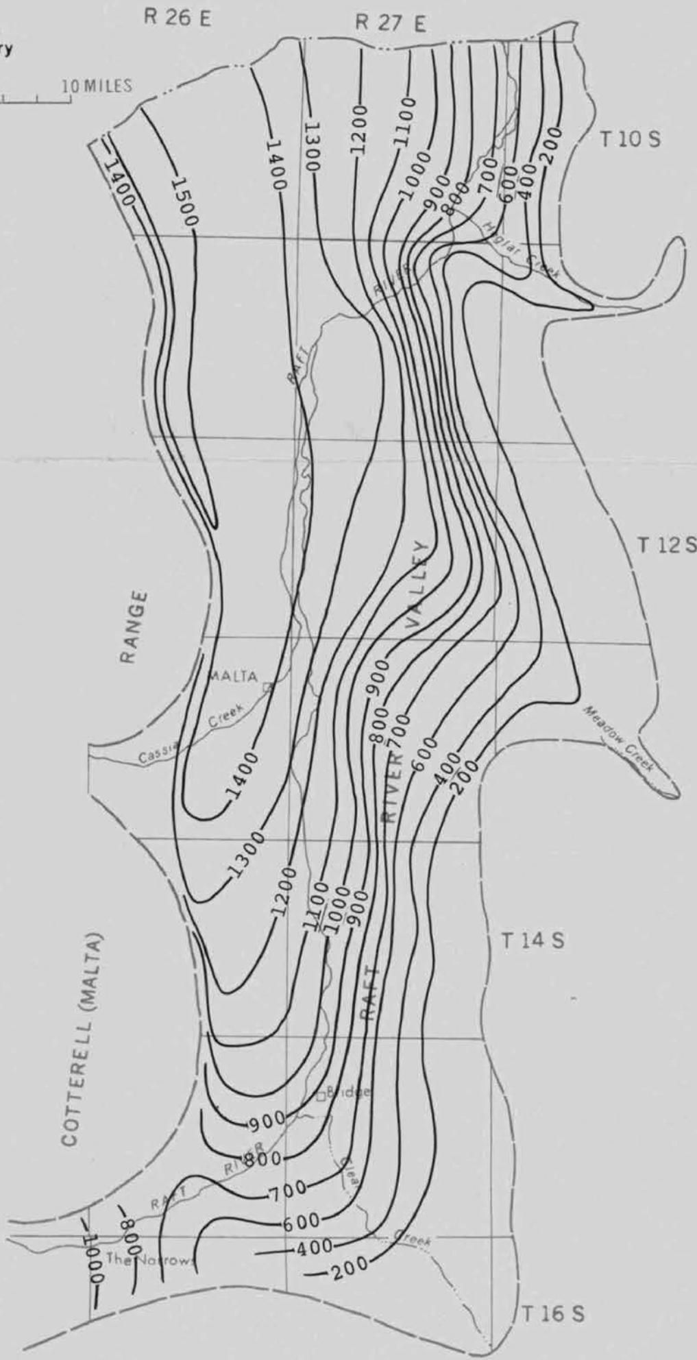
ALL PRINCIPAL WATER-BEARING DEPOSITS IN THE RAFT RIVER VALLEY SUBBASIN
