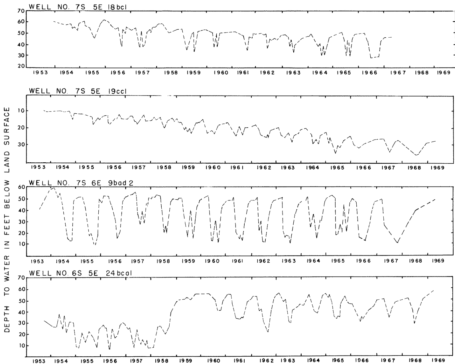
FIGURE 19. Hydrographs of wells 6S 5E 24bcal, 7S 5E 18bcl, 7S 5E 19cccl and 7S 6E 9badl in the Bruneau Subarea
