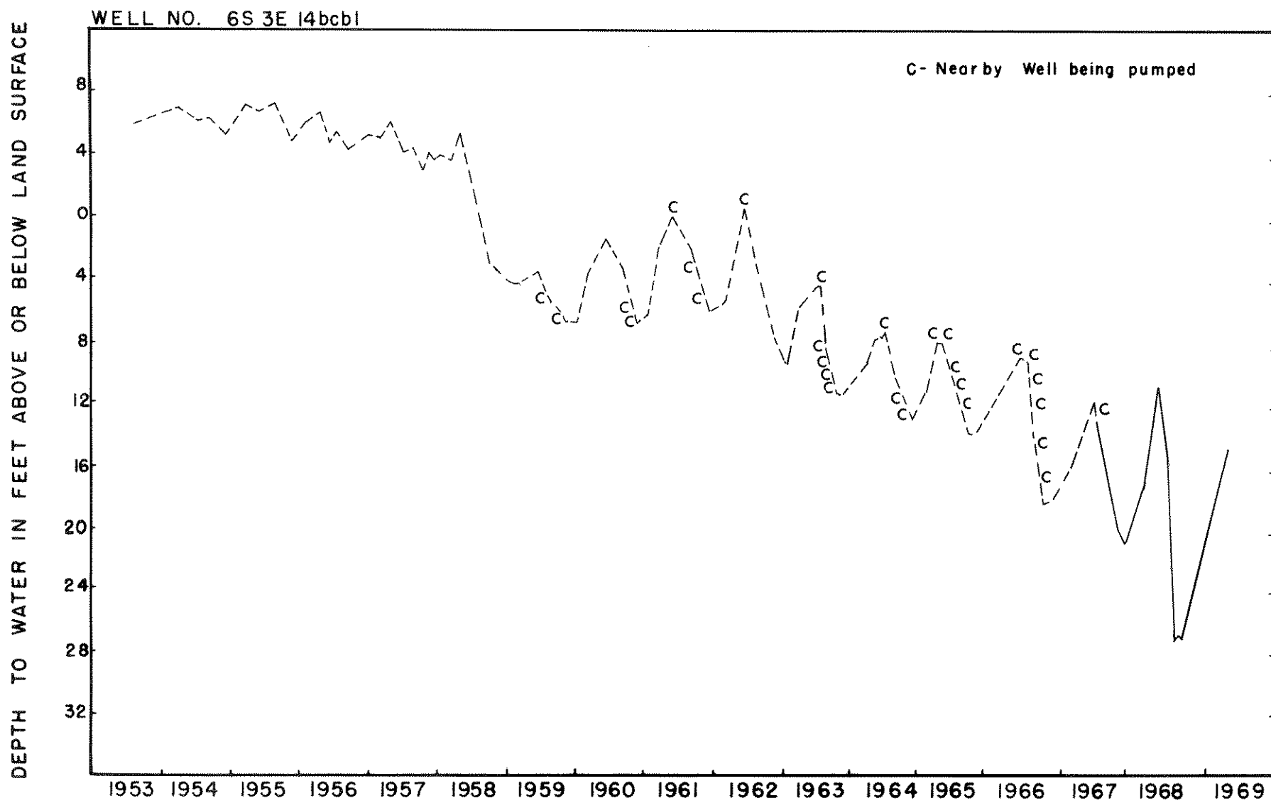
FIGURE 17. Hydrograph of well 6S 3E 14bcb in the Grand View Subarea
