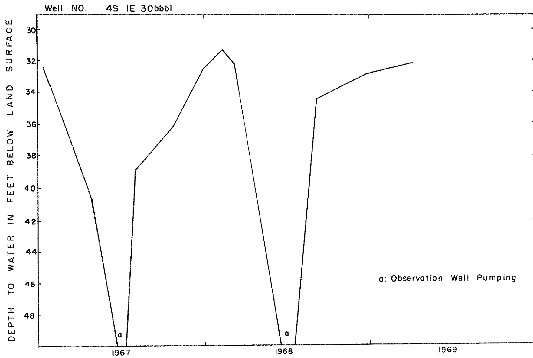
FIGURE 14. Hydrograph of well 4S 1E 30bb1 in the Oreana Subarea
