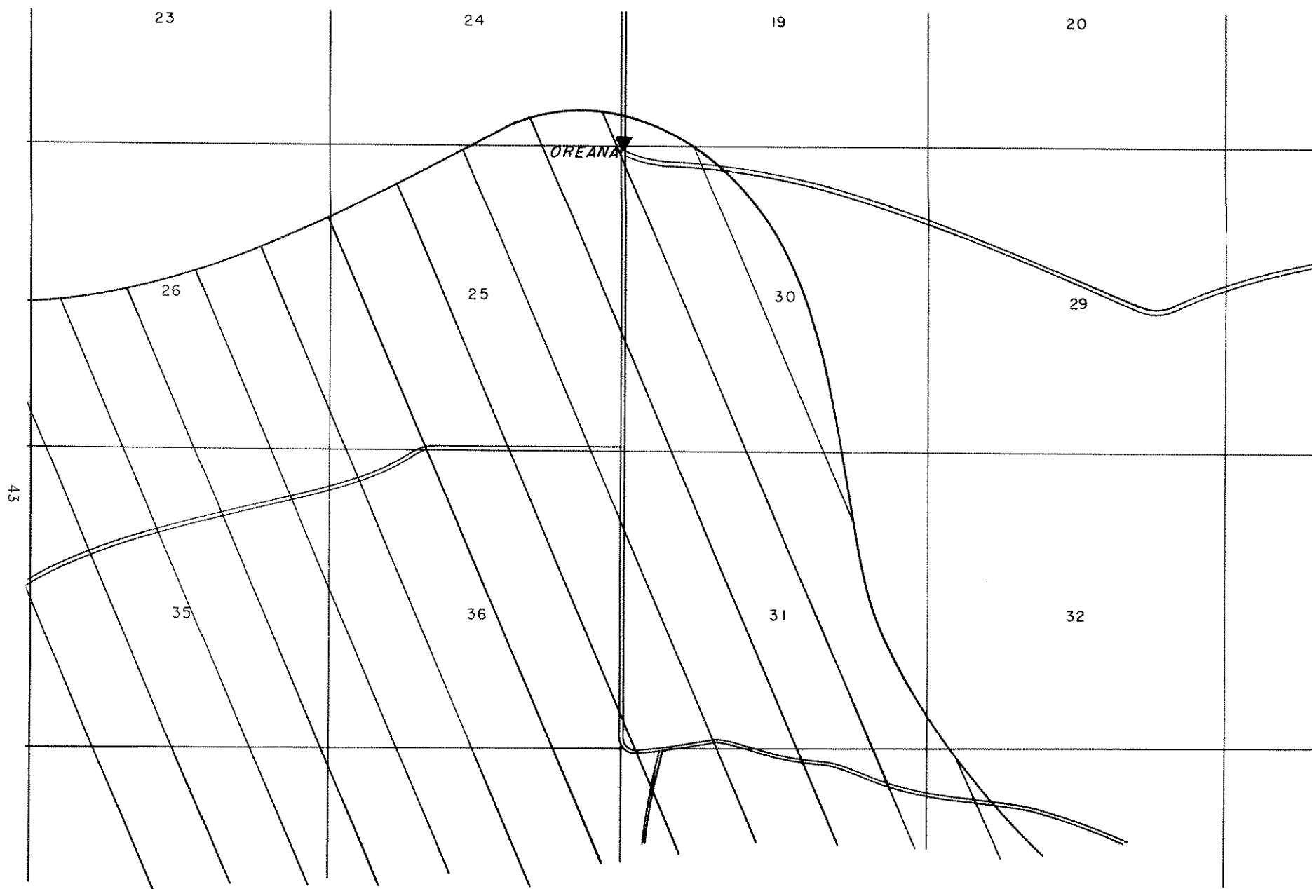
FIGURE 12. Extent of the sand aquifer in the Oreana area
