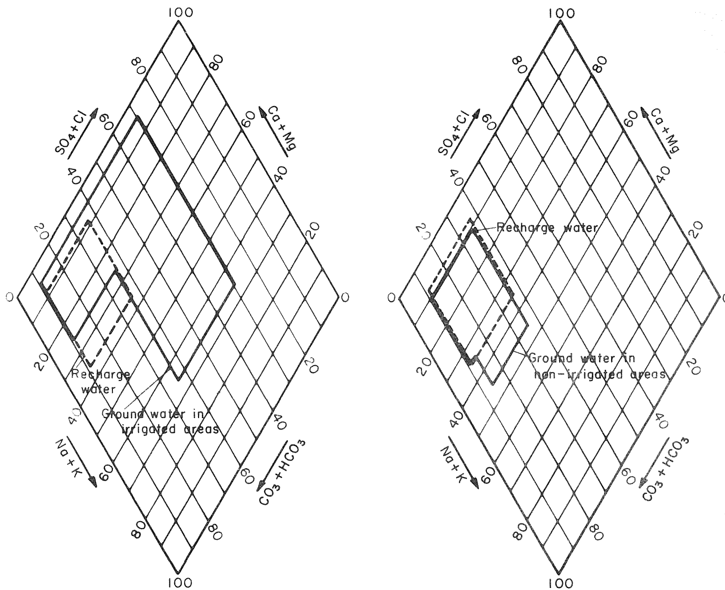
FIGURE 10.--Comparison of quality of recharge water and ground water. Blocks enclose ranges of compositions in percentages.
