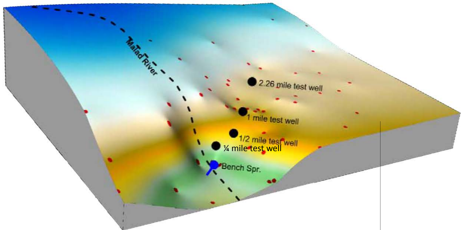
Figure 9. 3-D water table map with locations of tracer test wells in the same flow path. Note the steep water table around Malad Gorge where the 'Bench' spring is located. View angle is to the southeast.
