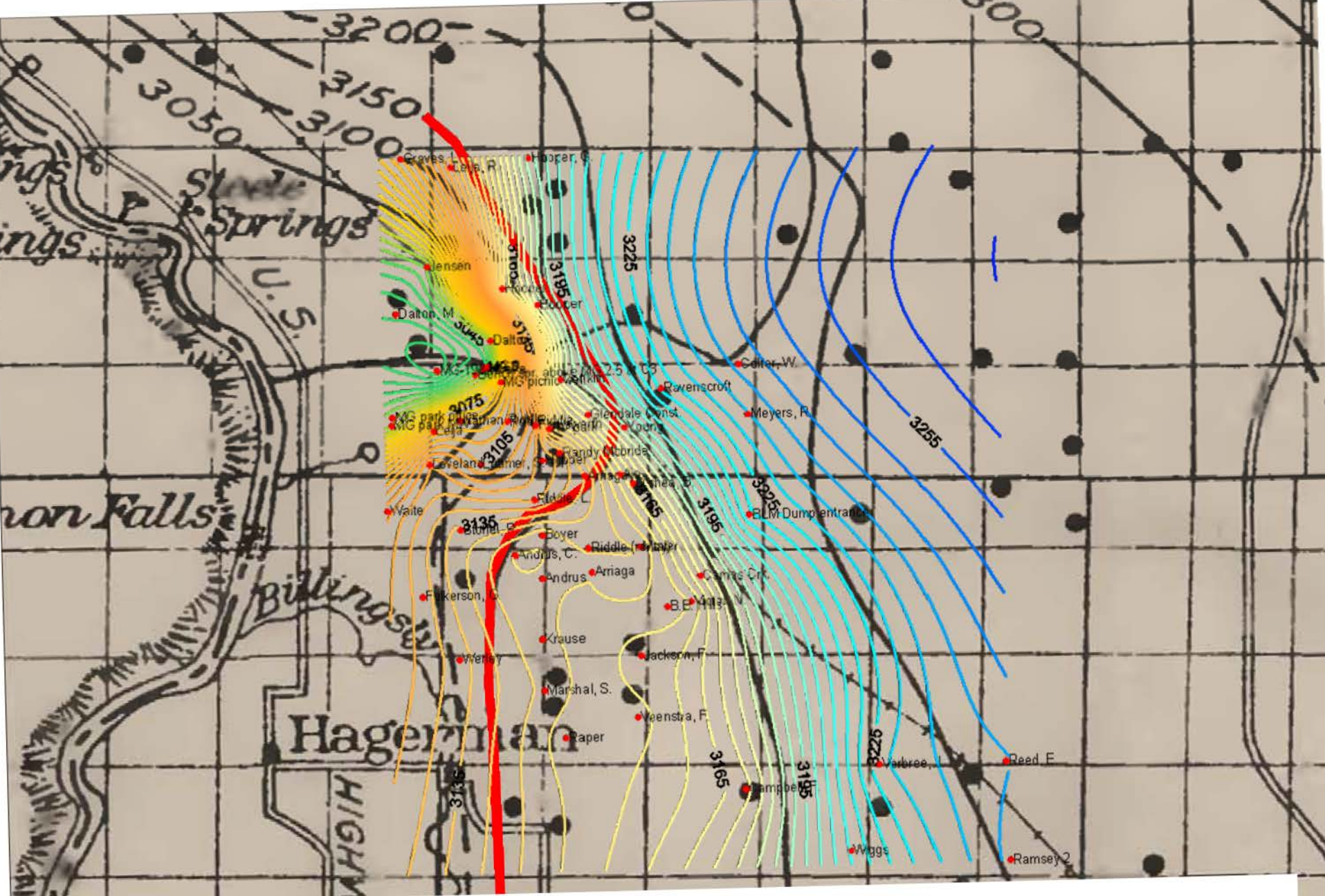
Figure 10. Groundwater contours from April 2011 shown with the color gradient overlain onto H.T. Stearns 1938 map. Note the concave then convex shape of the red highlighted contour from Stearn's map compared to the same patterns of the high resolution contours.
