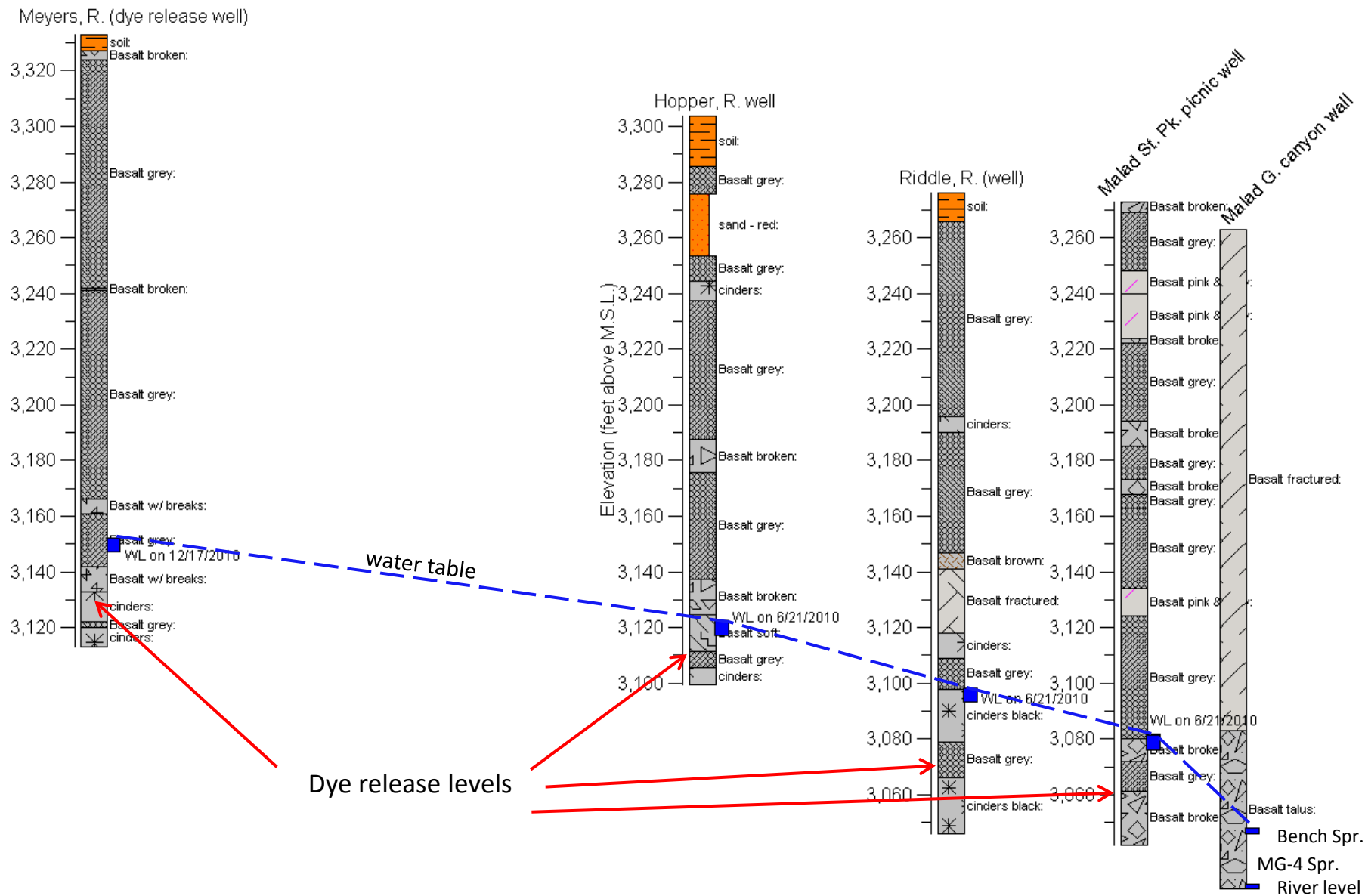
Figure 7. Geologic cross section of four wells and the Gorge wall showing elevations of dye release related to the geology and water table. The distance between the Meyer well and the Gorge is 2.26 miles. The Hopper well is about 1 mile and Riddle well about ½ mile.
