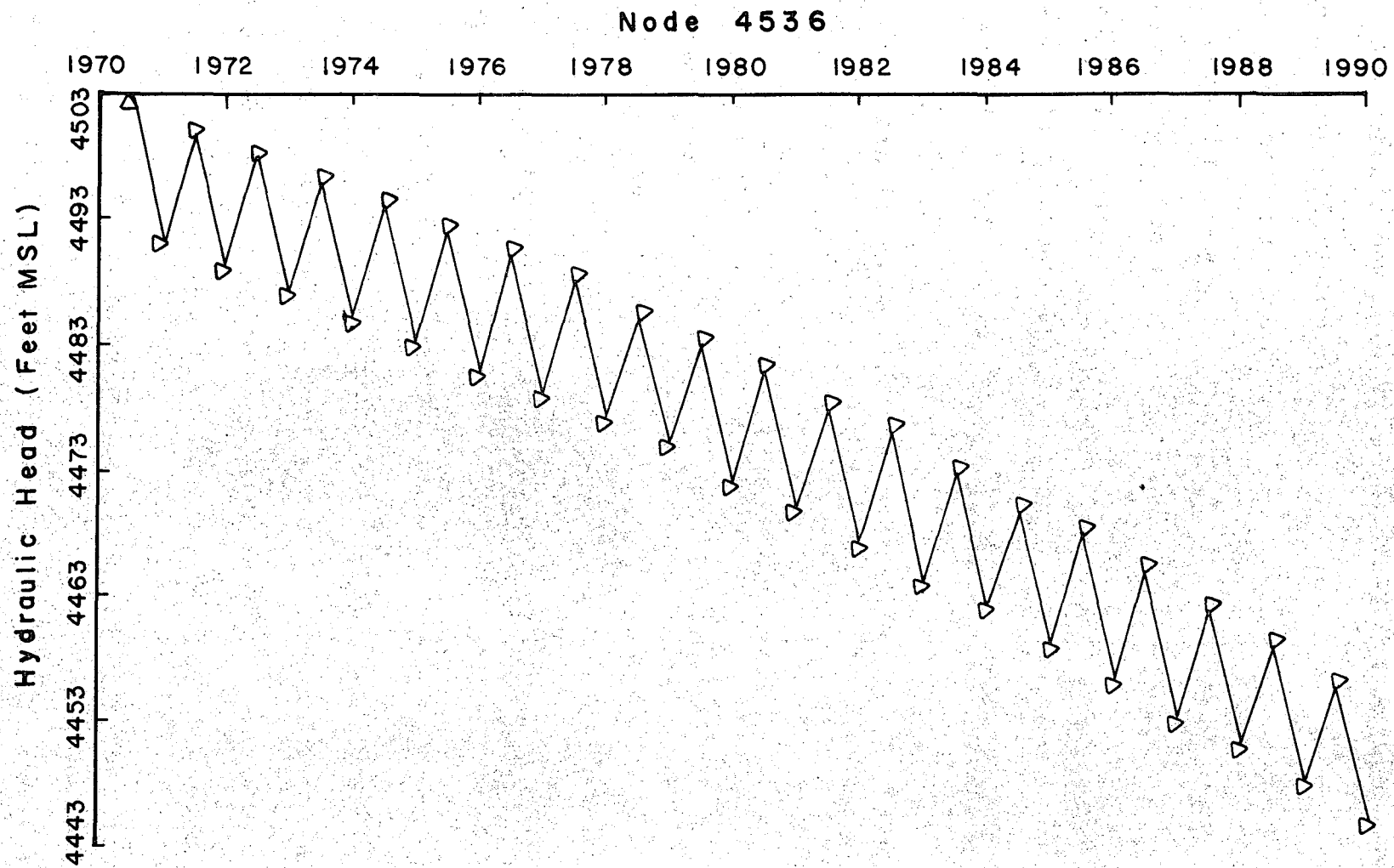
Figure 5 Hydrograph of the Well at Node 4536, Basis Run
