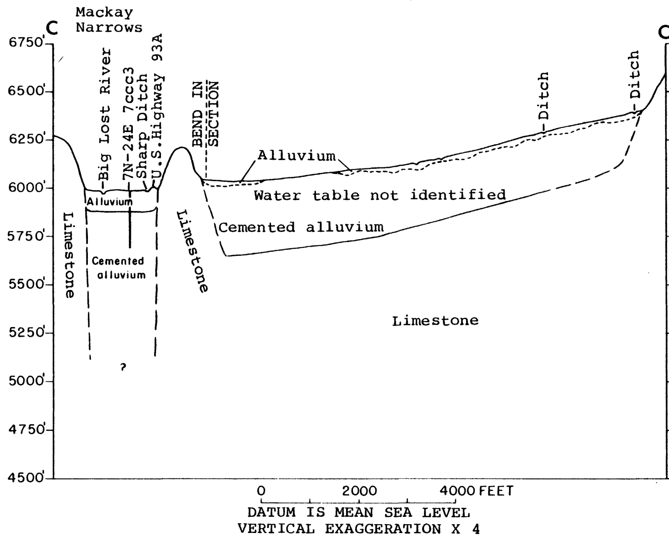
FIGURE 14.-- Geologic section C-C' across Big Lost River at Mackay Narrows, compiled from well logs, seismic data, and surficial geology. (See fig. 10 for location of section).
