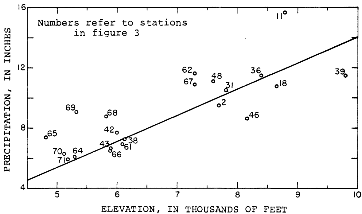
FIGURE 6.-- Precipitation-elevation relations in the Big Lost River area for the warm season of the 1967 water year.
