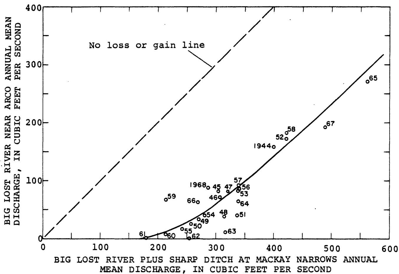
FIGURE 22.-- Relation between surface flow at Mackay Narrows and flow below Arco, 1944-68.
