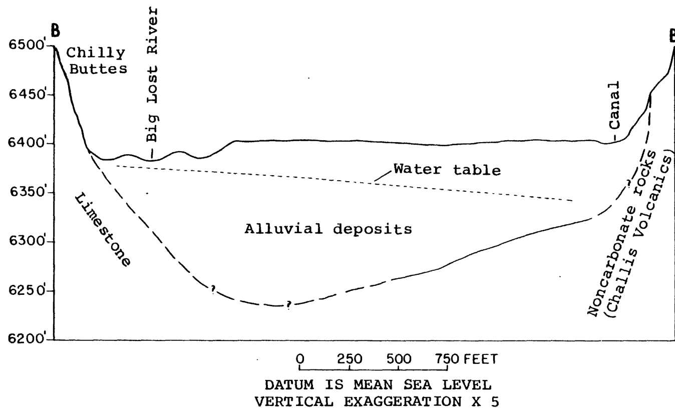
FIGURE 13,-- Geologic section B-B' across Big Lost River valley at Chilly Buttes based on seismic data. (See fig. 10 for location of section).
