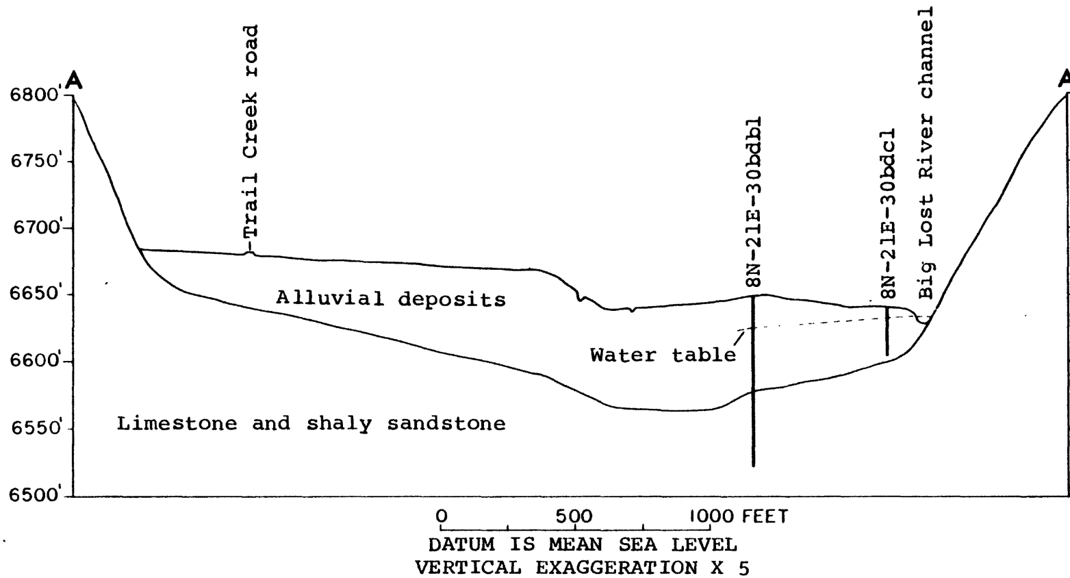
FIGURE 12.-- Geologic section A-A' near Howell Ranch compiled from well logs and seismic data. (See fig. 10 for location of section)
