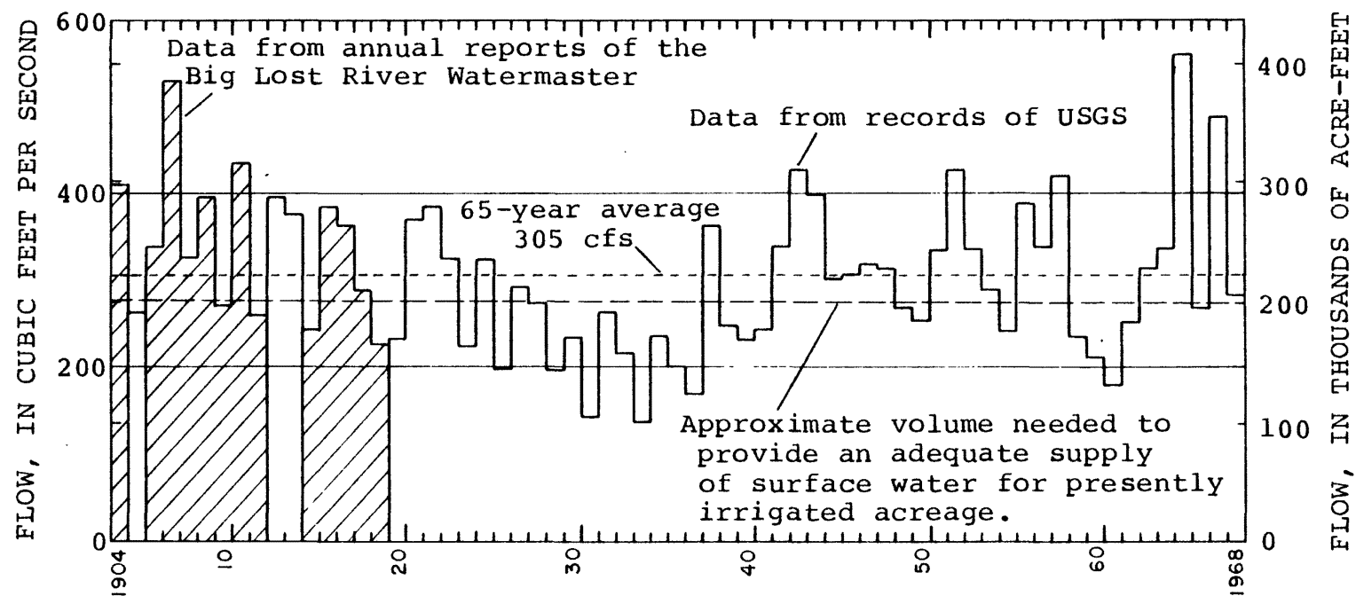
FIGURE 29.-- Flow of Big Lost River at Mackay Narrows. (Big Lost River near Mackay and Sharp Ditch near Mackay).
