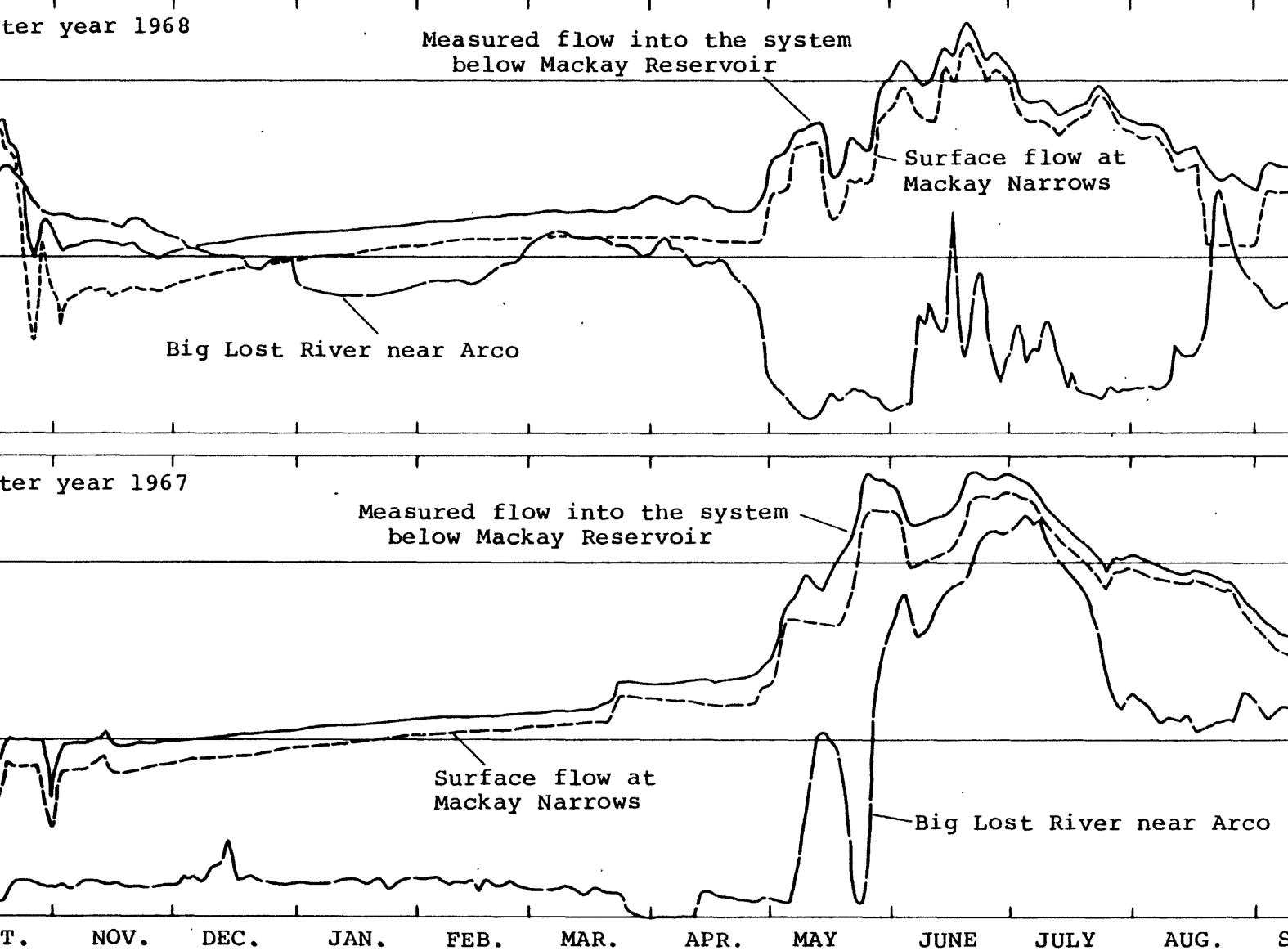
FIGURE 21.-- Hydrographs of surface flow below Mackay Narrows.
