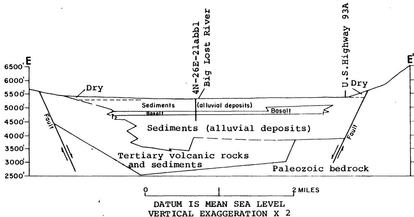
FIGURE 15.-- Generalized geologic section E-E' north of Arco compiled from gravity, seismic-refraction, and resistivity surveys. By Mabey, Zohdy, Peterson, and Mattick, 1969 personal communication. (See fig. 10 for location of section).
