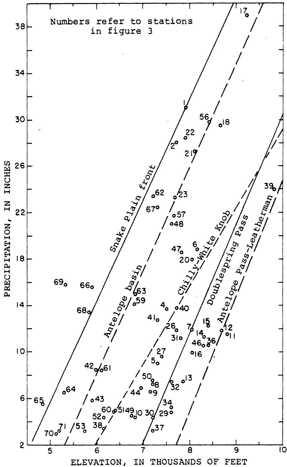
FIGURE 7.-- Precipitation-elevation relations in the Big Lost River area for the cold season of the 1967 water year.
