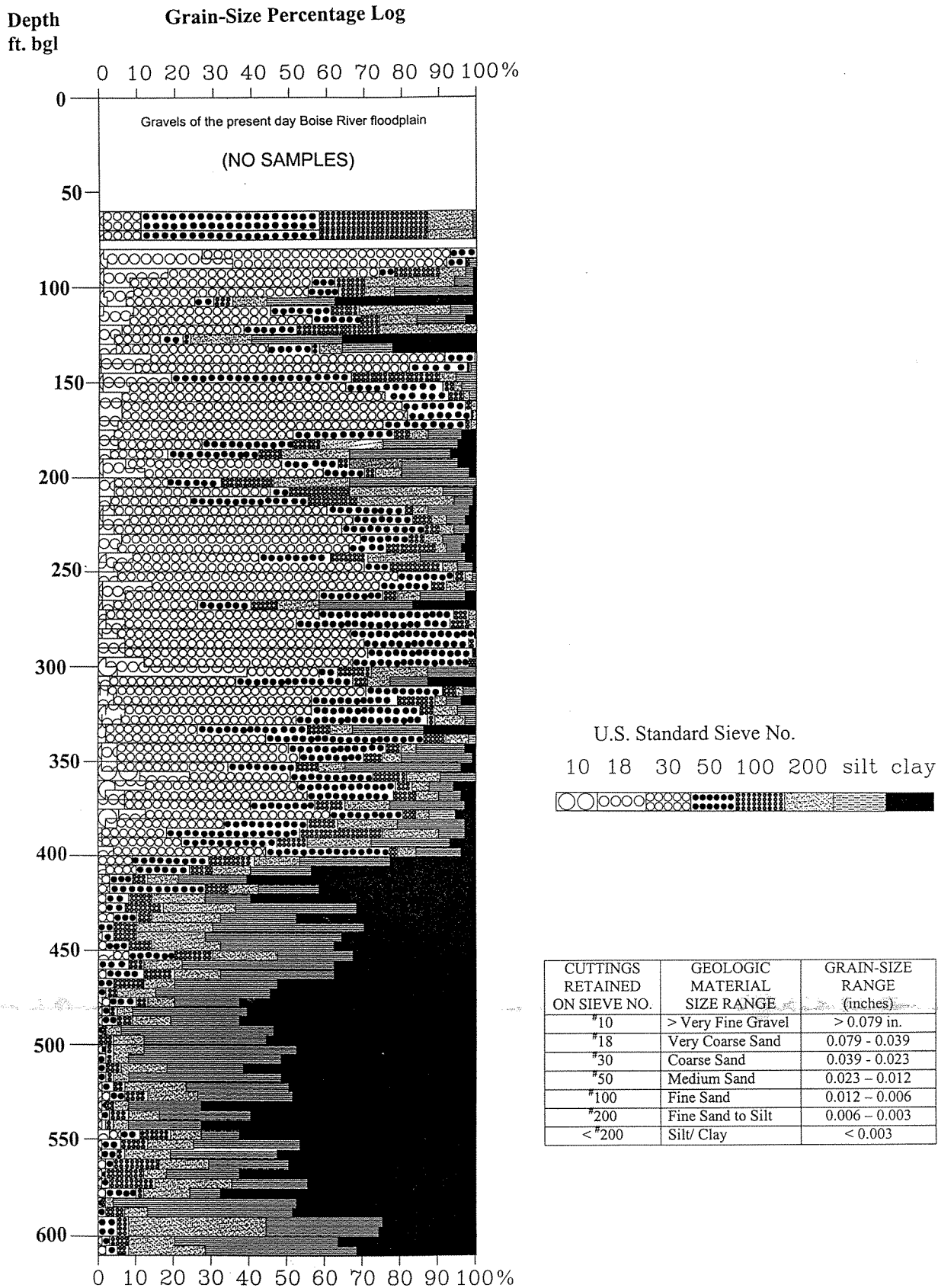
Figure 4. Grain-size percentage log of drill-cuttings from the TVHP #1 test-well. Each five-foot sample interval was wet-washed through a stack of U.S. Standard sieves and the relative percentages retained, by volume, were measured. The silt and clay fractions were estimated by settling the wash-through water, and delineated from one another by setting time in a graduated cylinder. Sieve analysis by Boise State University graduate students Brian Cavanagh and Mike Guilbert of the Department of Geosciences. The log is meant to be an objective representation of grain size distribution with depth, however, recirculated sand, cavings, and the loss of clay and silt particles in the drill-cuttings can affect the log. The log cannot be directly correlated with geophysical logs owing to the cuttings return "lag time".
