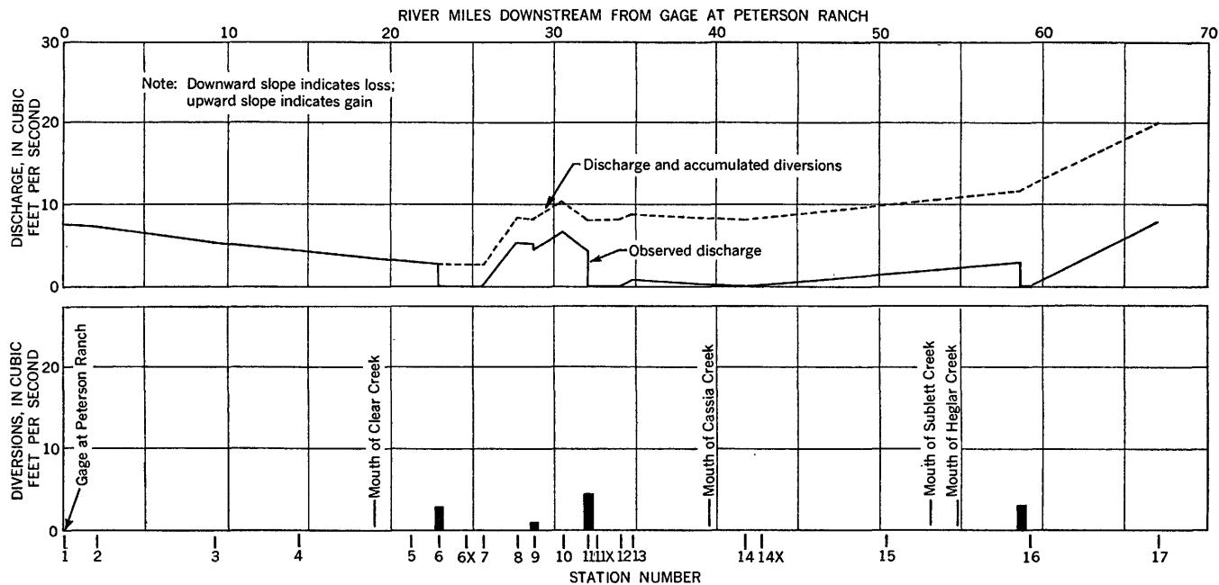
FIGURE 13.—Losses, gains, and diversions of Raft River below Peterson Ranch, July 31–August 2, 1950.
