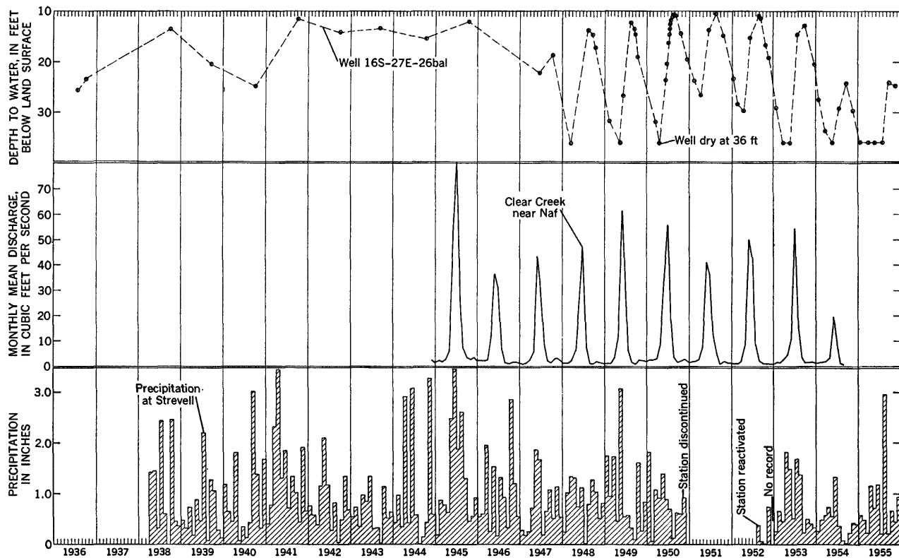
FIGURE 17.—Hydrograph of well 16S-27E-26a1, and Clear Creek near Naf, compared with precipitation and runoff.
