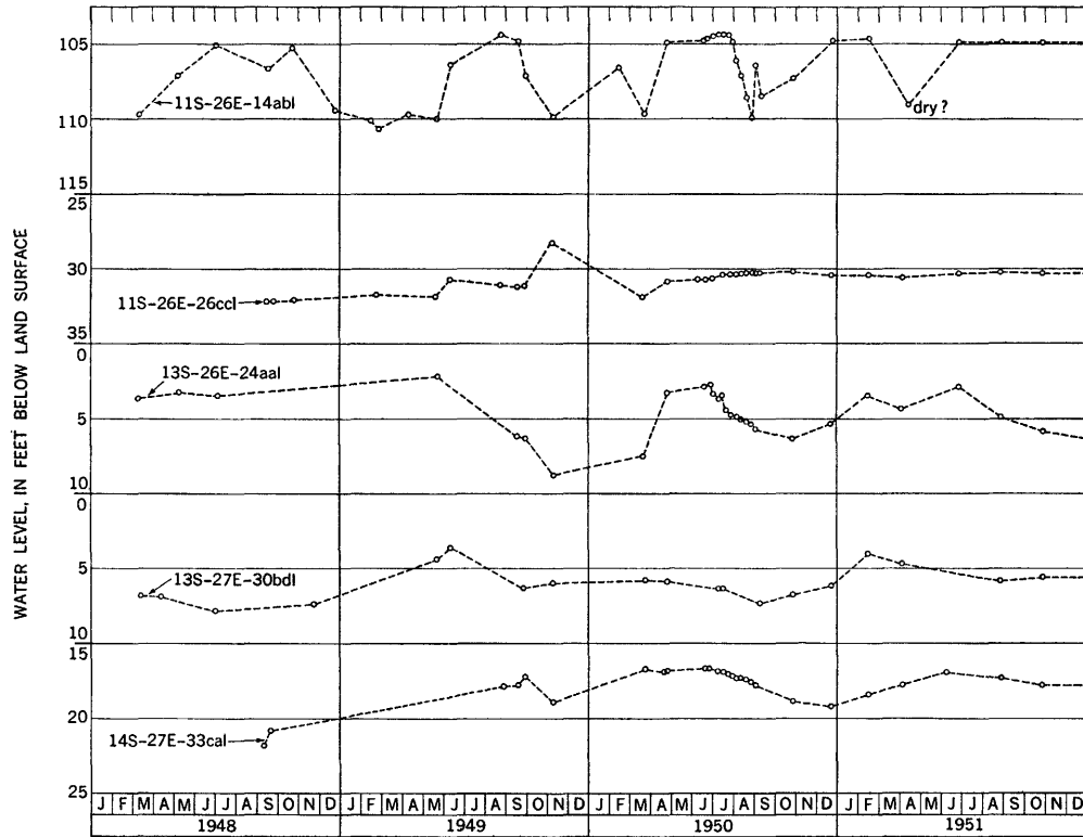
FIGURE 14.—Hydrographs of wells in the Raft River valley, 1948-51.
