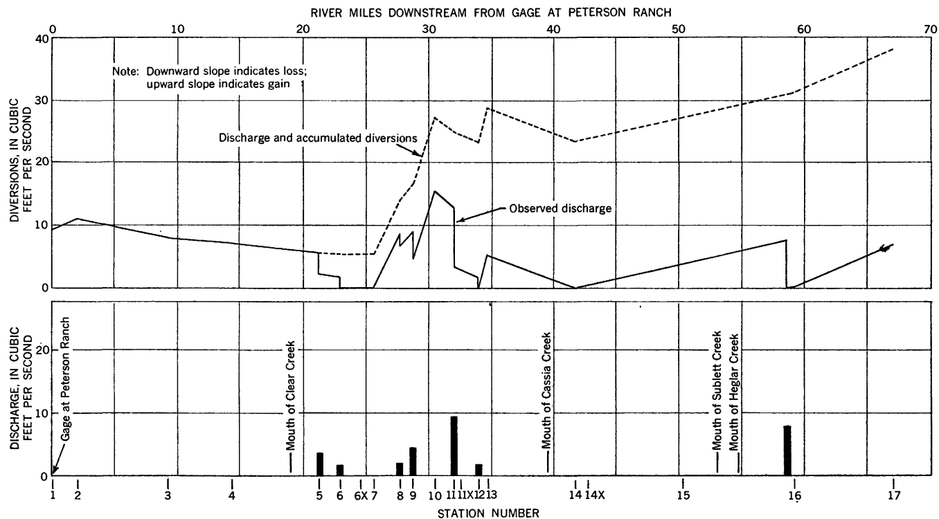
FIGURE 12.—Losses, gains, and diversions of Raft River below Peterson Ranch, June 28–July 5, 1950.
