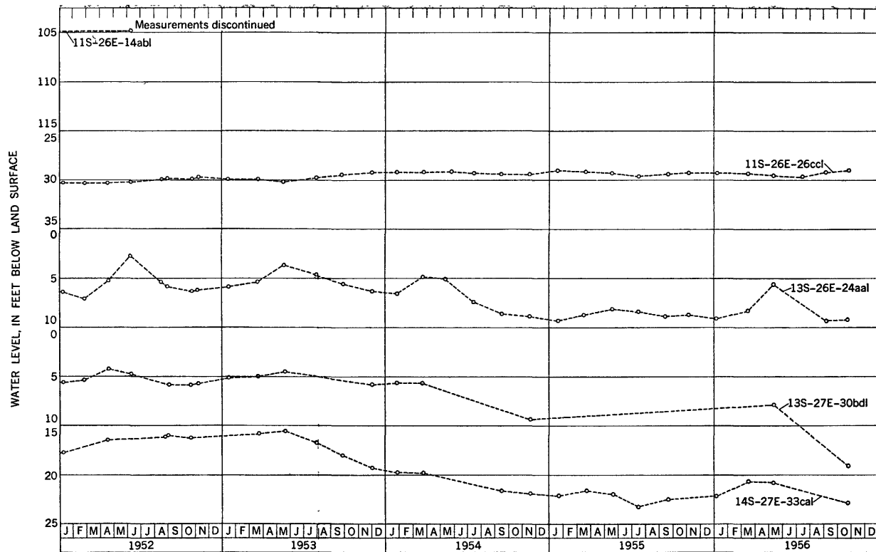
FIGURE 15.—Hydrographs of wells in the Raft River valley, 1952-56.
