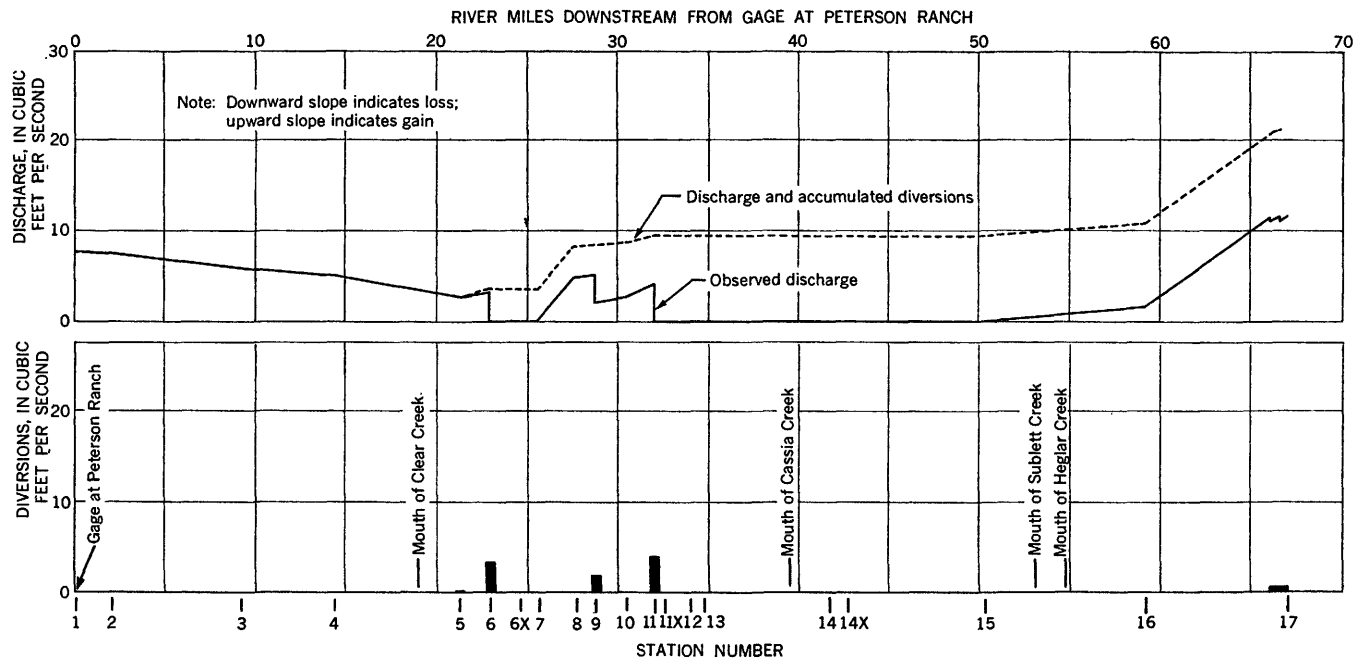
FIGURE 10.—Losses, gains, and diversions of Raft River below Peterson Ranch, September 13–20, 1949.
