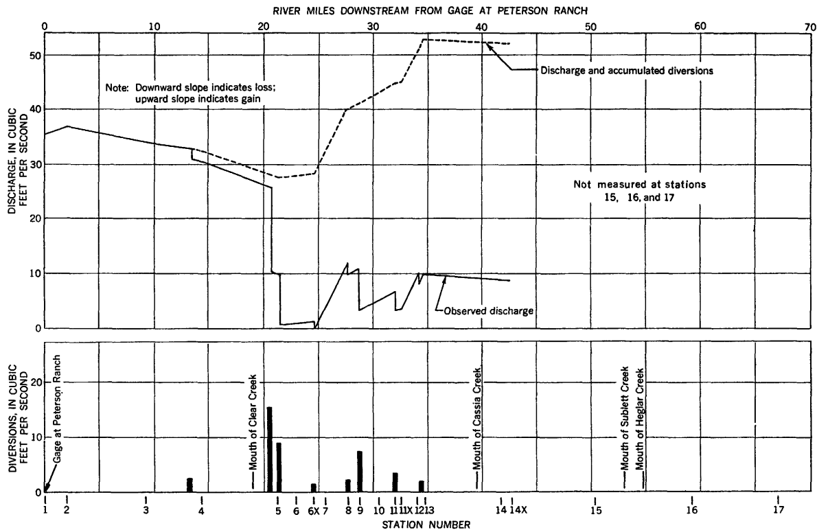
FIGURE 11.—Losses, gains, and diversions of Raft River below Peterson Ranch, April 24–26, 1950.
