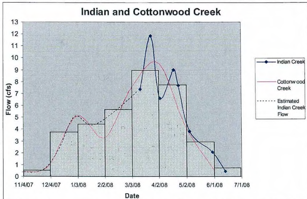
Figure 3. Hydrographs of Indian Creek and Cottonwood Creek. The runoff volume in Indian Creek was estimated by summing the areas of the shaded rectangles. Cottonwood Creek hydrograph was downloaded from http://waterdata.usgs.gov/nwis/sw .
