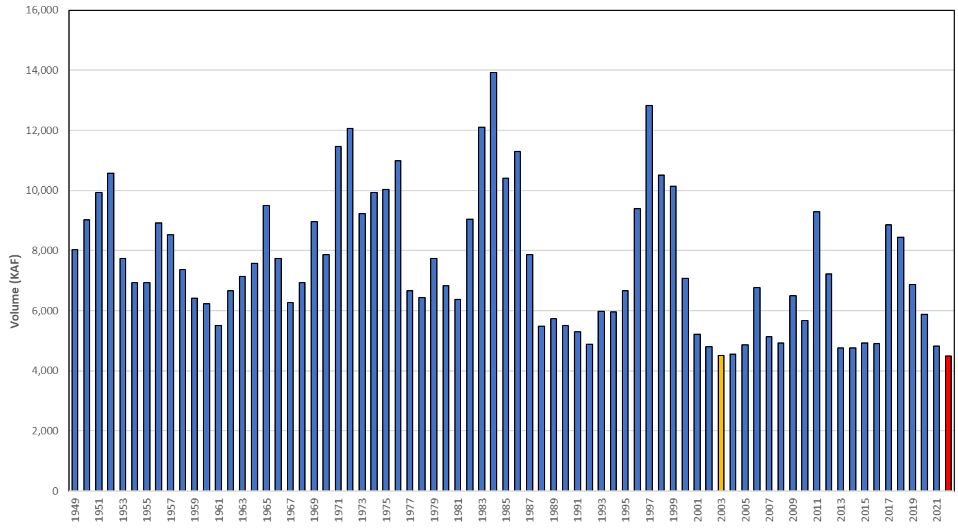
Snake River nr Murphy Water Year Observed Volume (Oct-Sep)
