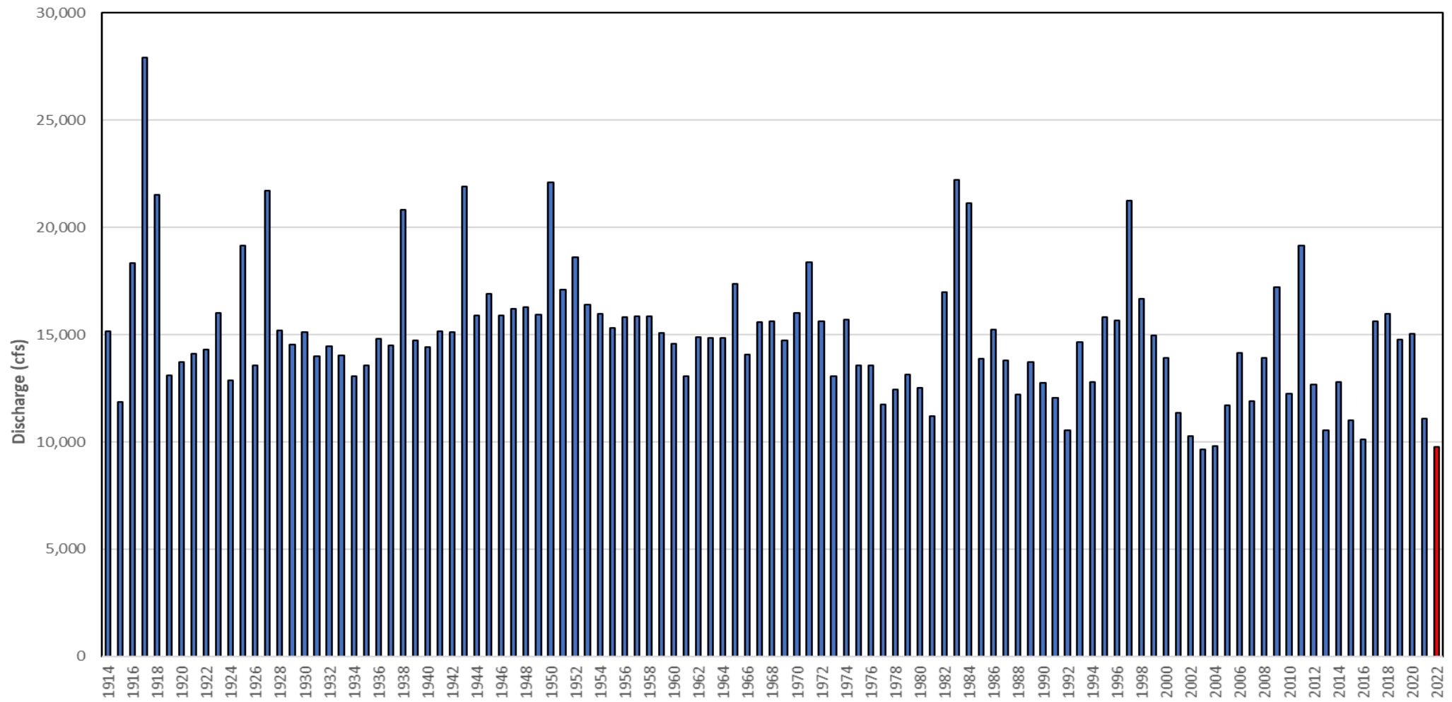
Snake River nr Murphy July Average Plus August Average Discharge
