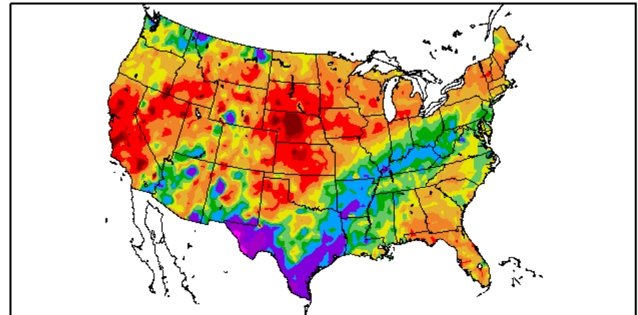
Percent of Normal Precipitation (%) 3/1/2015 – 3/31/2015
