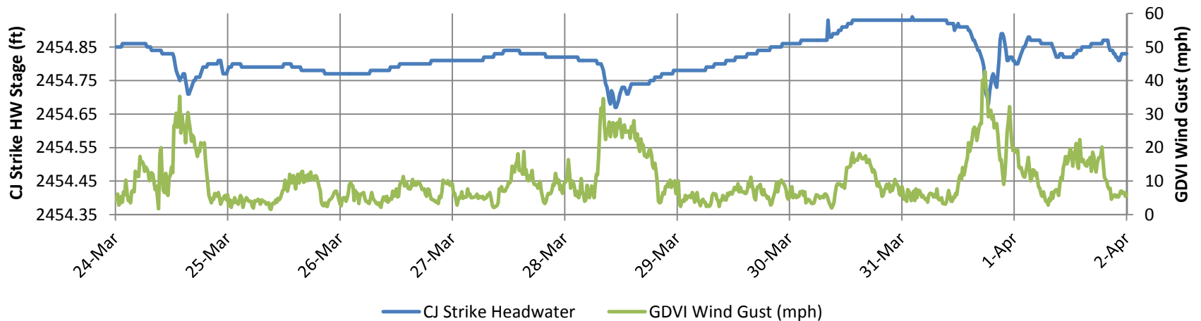
CJ Strike Headwater and Wind at GDVI
