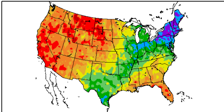
Departure from Normal Temperature (F) 3/1/2015 – 3/31/2015
