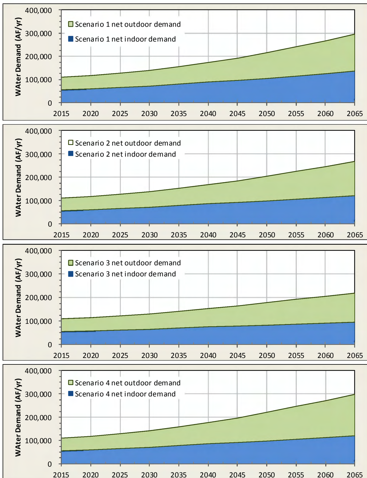
Figure 40. DCMI water-demand projections, Scenarios 1-4.
