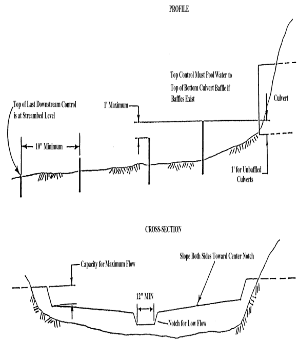
FIGURE 18. Downstream Control Structures Used to Reduce Downstream Erosion and Improve Fish Passage
