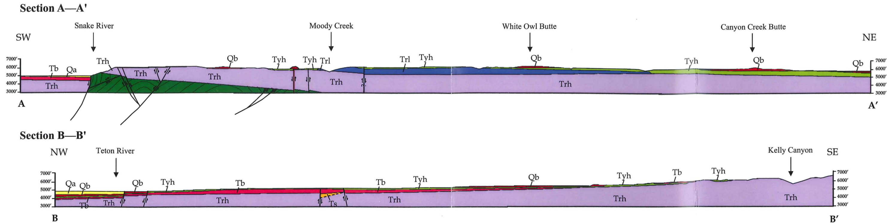
Figure 1 Geologic Cross Sections
