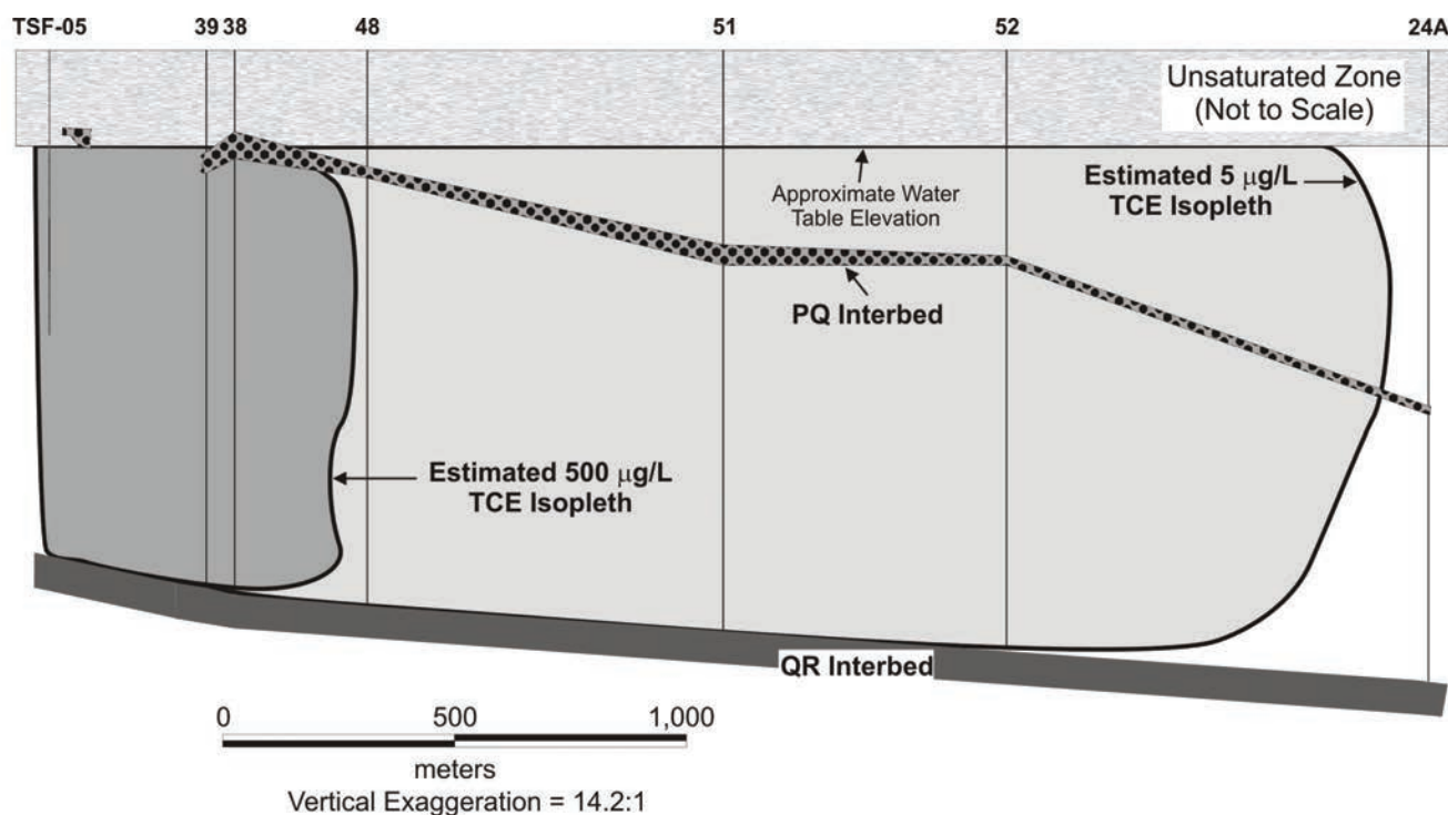
Figure 3-7. Conceptual model cross-section at the scale of the TCE plume fringe.
