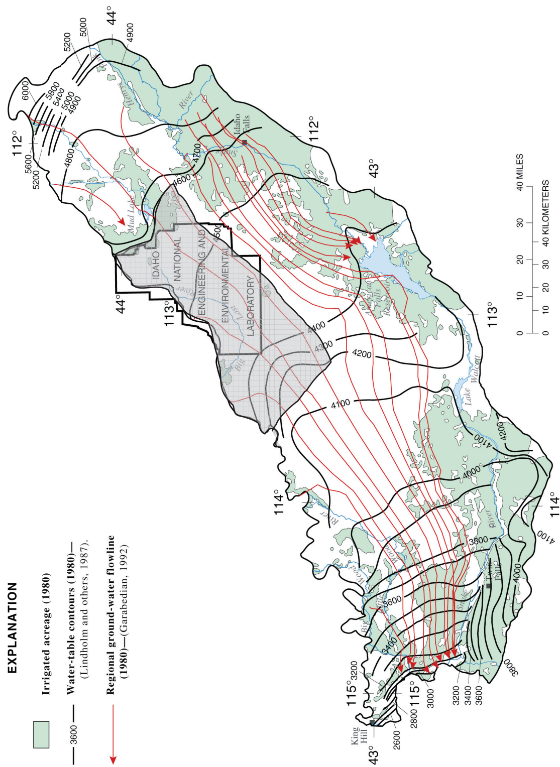
Figure 2-2. Extent of the USGS INEEL subregional conceptual model, eastern SRPA, Idaho (From Ackerman et al. in preparation).
