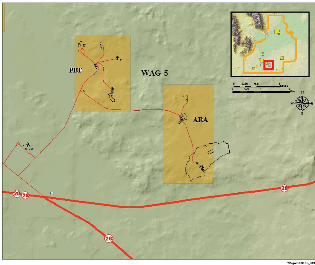
Figure 3-22. WAG 5 is associated with the ARA and the PBF in the south-central part of the INEEL.
