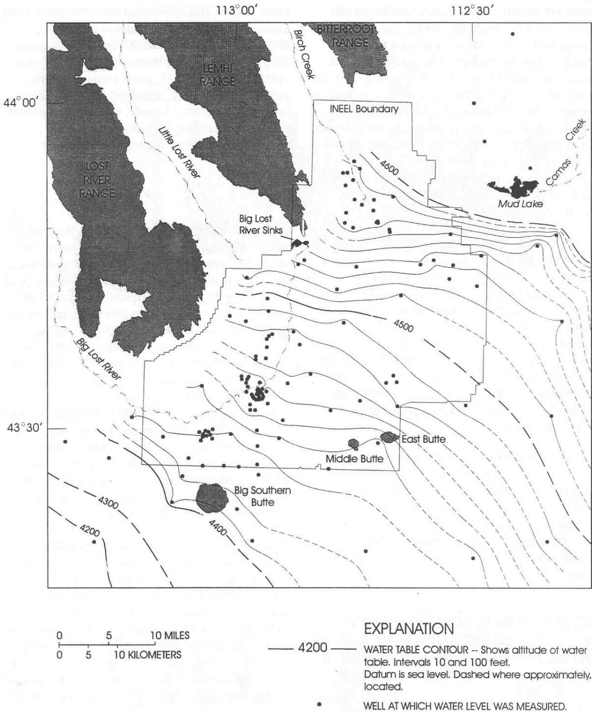
Figure 2-8. Altitude of the water table in the SRPA in the vicinity of the INEEL, 1998 (from Bartholomay et al. 2000).
