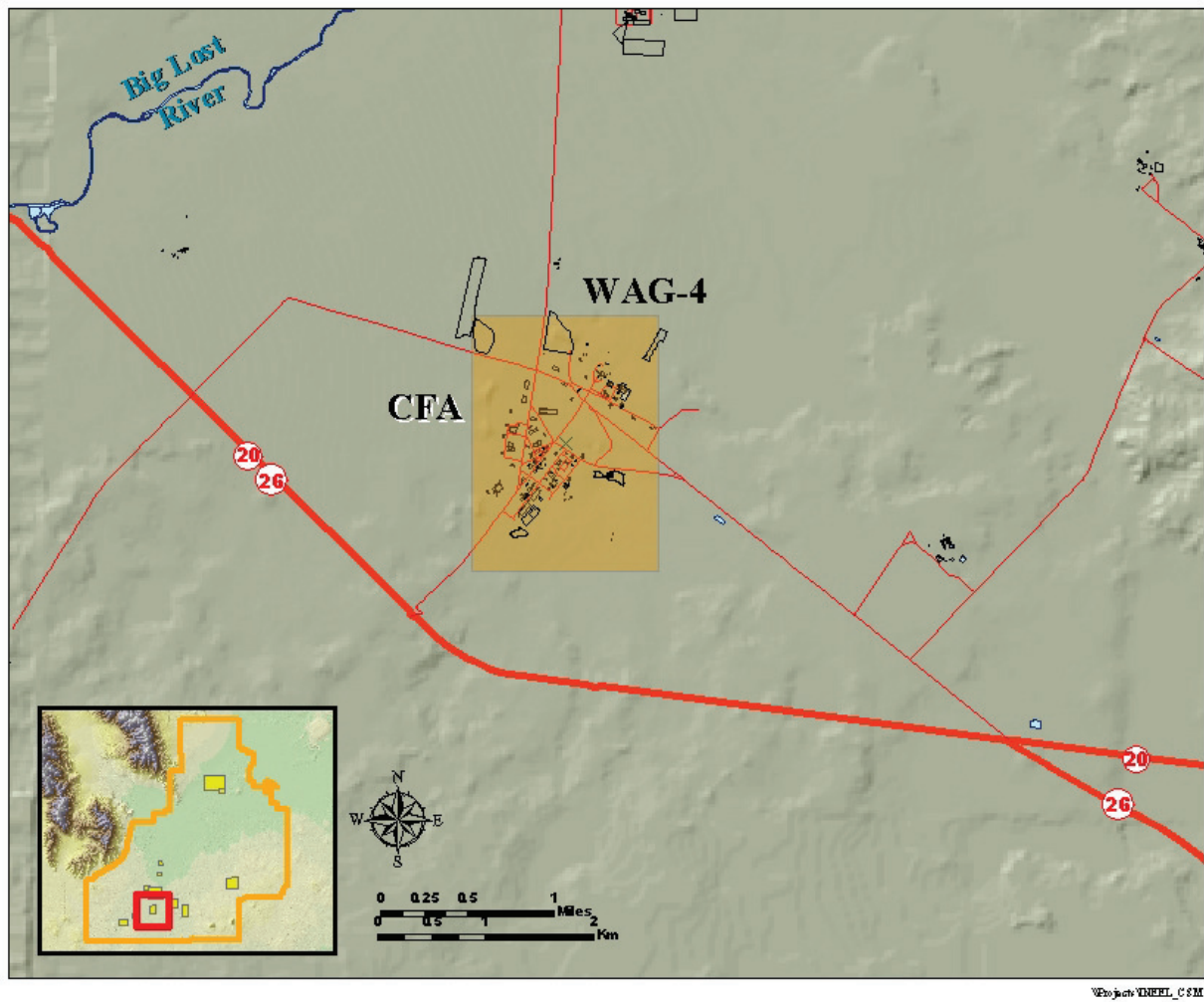
Figure 3-18. WAG 4 is associated with the CFA in the south-central part of the INEEL.
