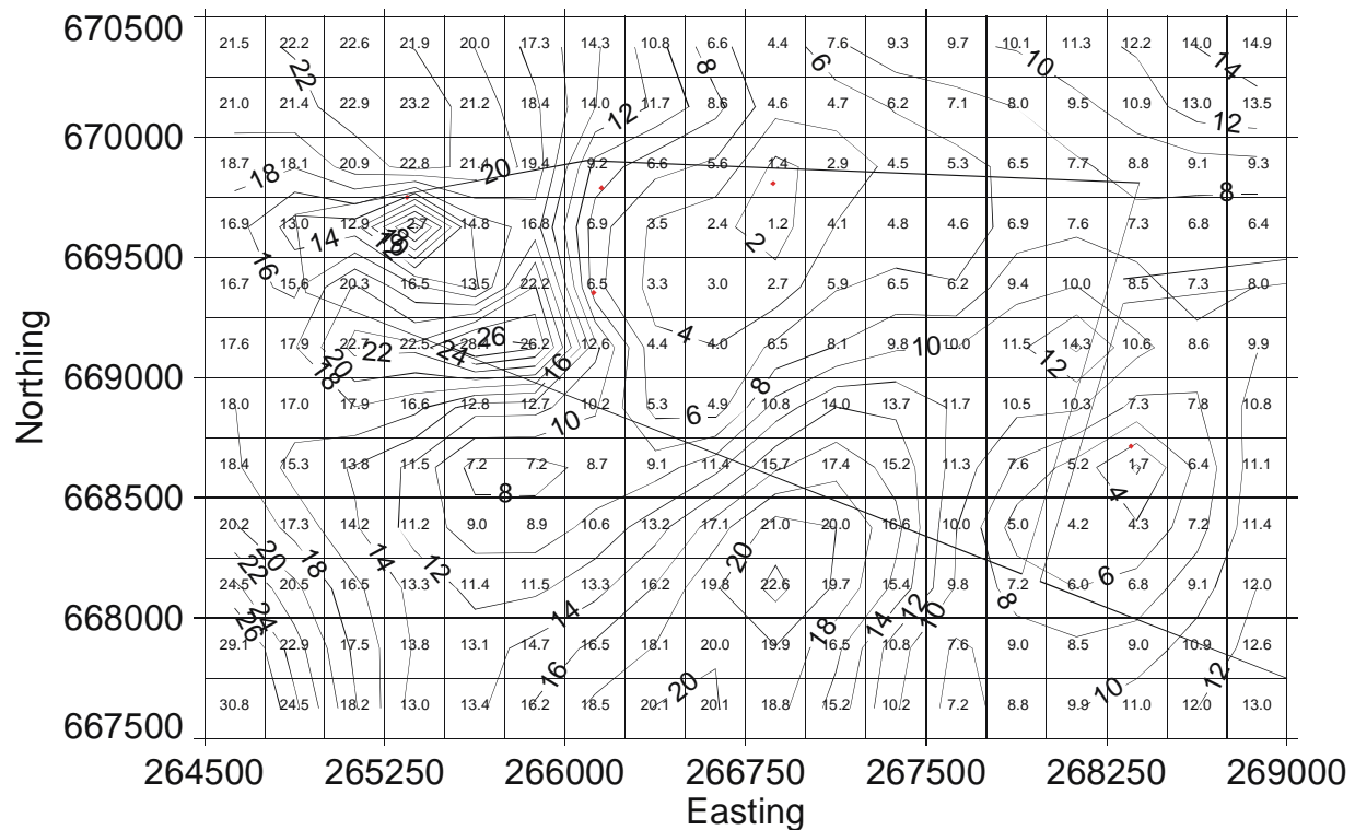
Figure 3-31. Kriged thickness results for the B-C interbed (adapted from Holdren et al. 2002). Interbed thickness is considered to be spatially variable. The lower plot includes the matrix of recent kriging results.
