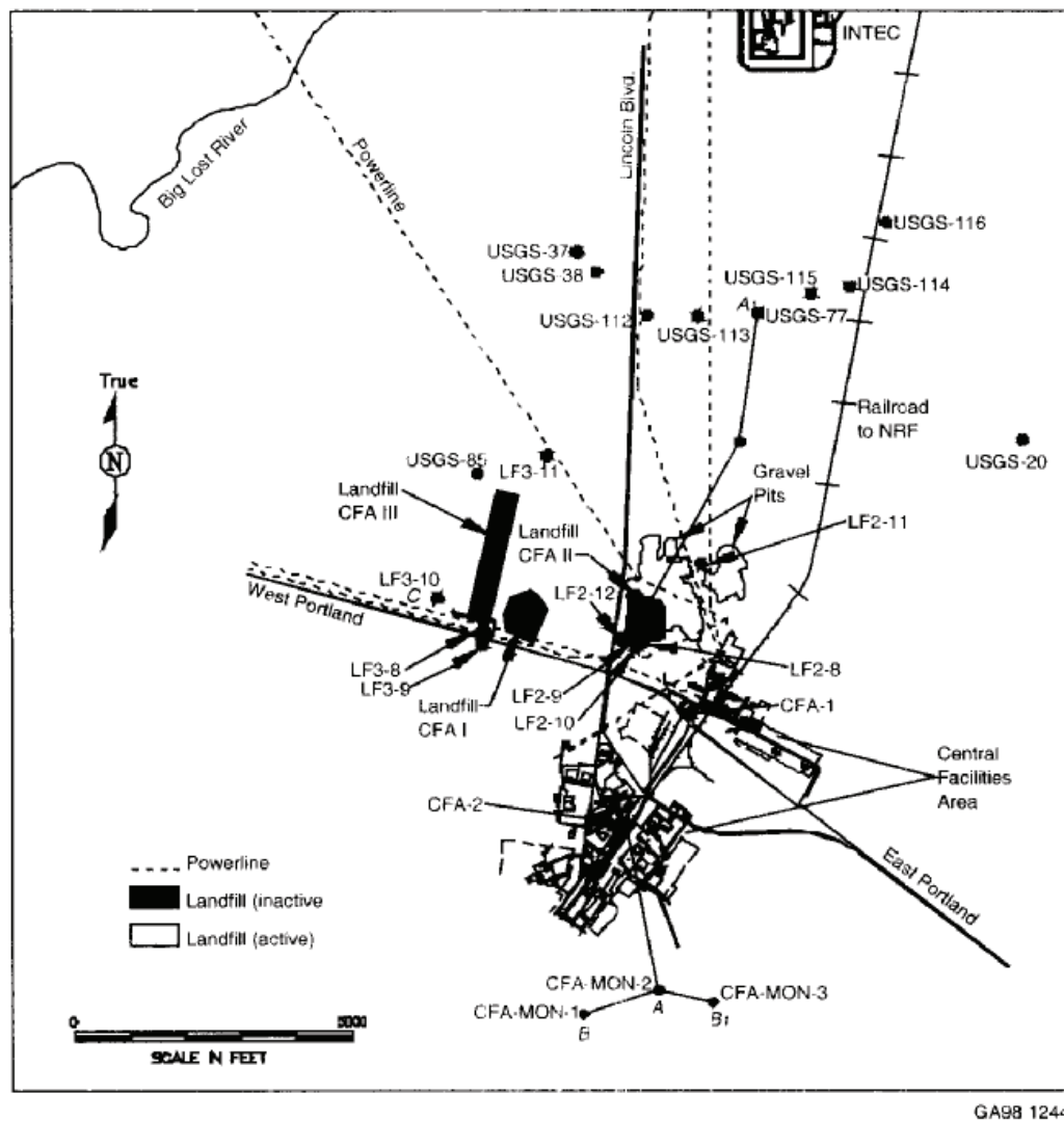
Figure 3-19. Well map for CFA area indicating stratigraphic cross section lines (adapted from Burgess et al. 2000).
