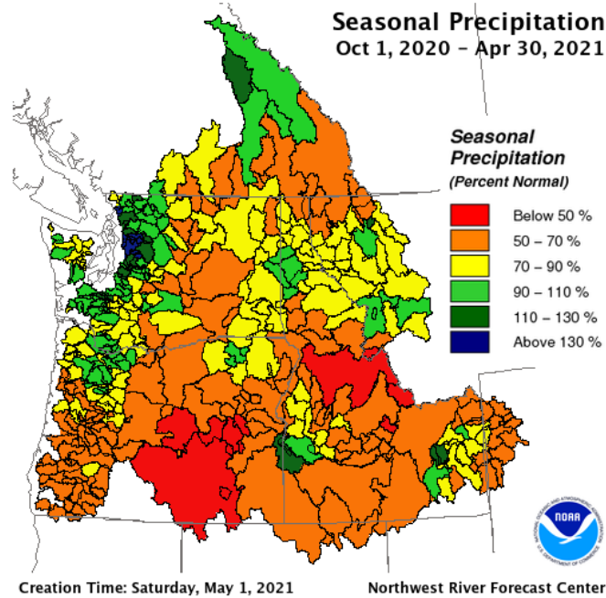
Figure 4: Seasonal Precipitation (Oct 1, 2020–April 30, 2021) for the Pacific Northwest (figure by the Northwest River Forecast Center) shows below normal seasonal precipitation across most of the basin with a few sub-basins near normal.
