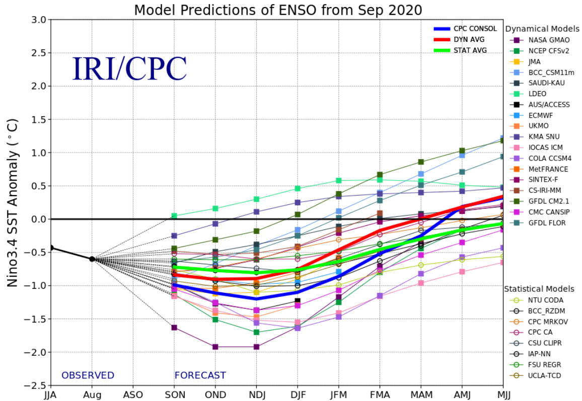
Figure 3: ENSO forecast plume from the International Research Institute for Climate and Society and the NOAA Climate Prediction Center showing the ENSO forecast during the fall of 2020.
