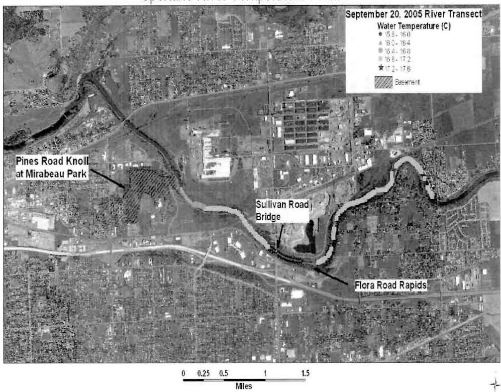
Figure 2 Temperature Readings Every 30 Seconds Spokane River Temperature Profile
