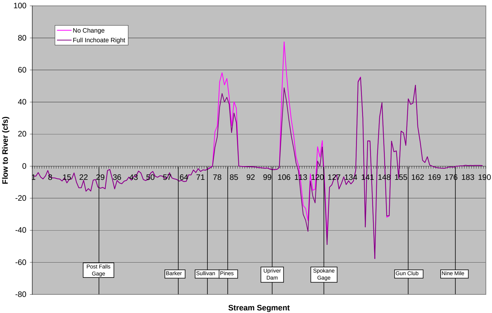
Figure 6: Aquifer/River Interaction - August 2005
