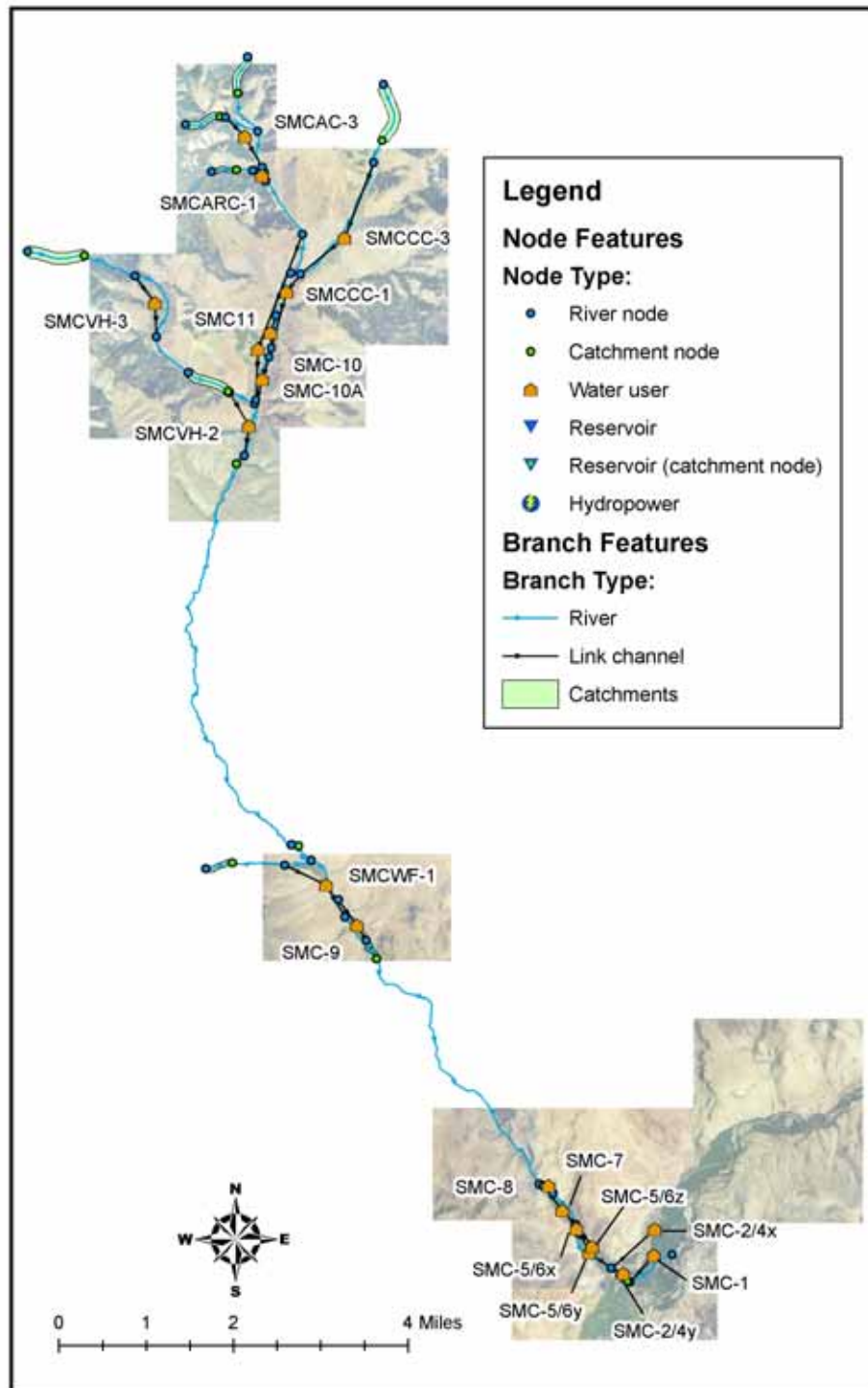
Figure 2. The MCMBM network. Blue lines represent streams and select ditches. Blue circles on the stream lines represent locations of offtake nodes or computational points and green circles represent the downstream extent of catchment areas. Orange pentagons represent irrigation nodes and thin black represent connections between the river and irrigation nodes. Note the thin black and green lines do not follow the exact path of ditches.
