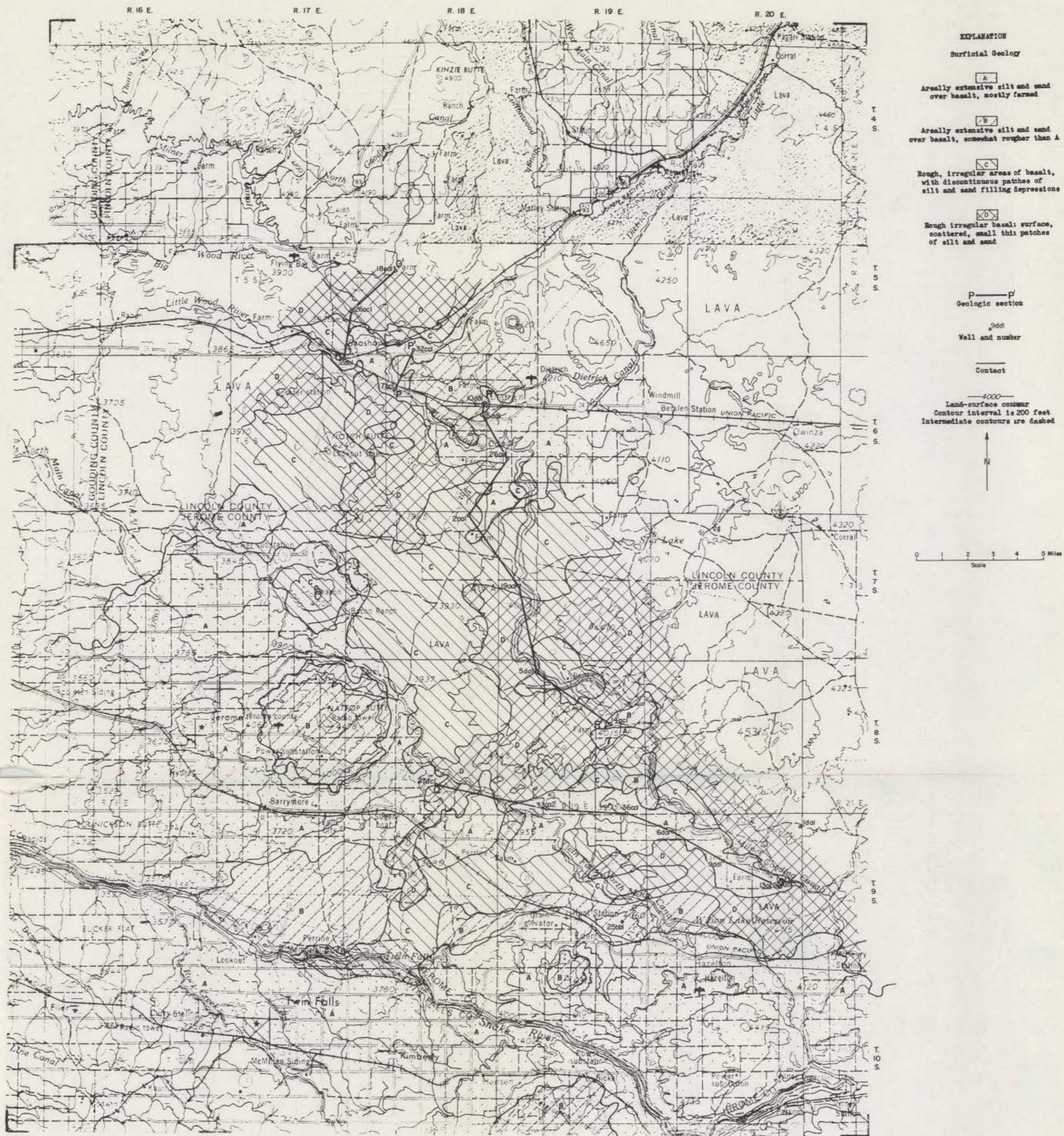
Figure 42.—Map of Milner-Shoshone area showing geologic features relating to recharge feasibility.
