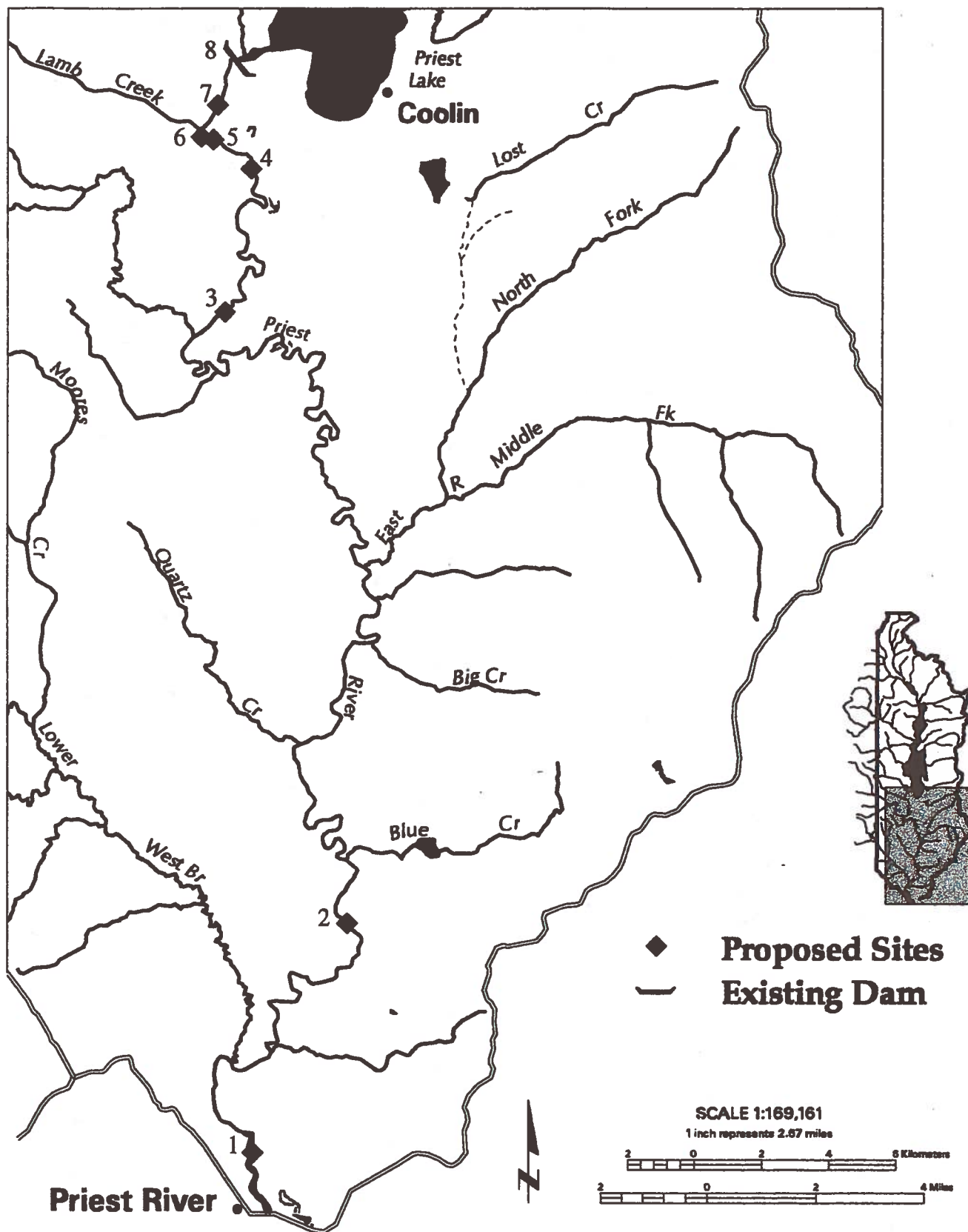
Figure 8. Hydroelectric Sites
