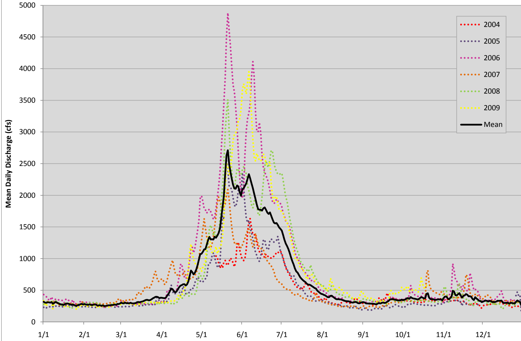
Salmon River Flows near Stanley 2004-2009
