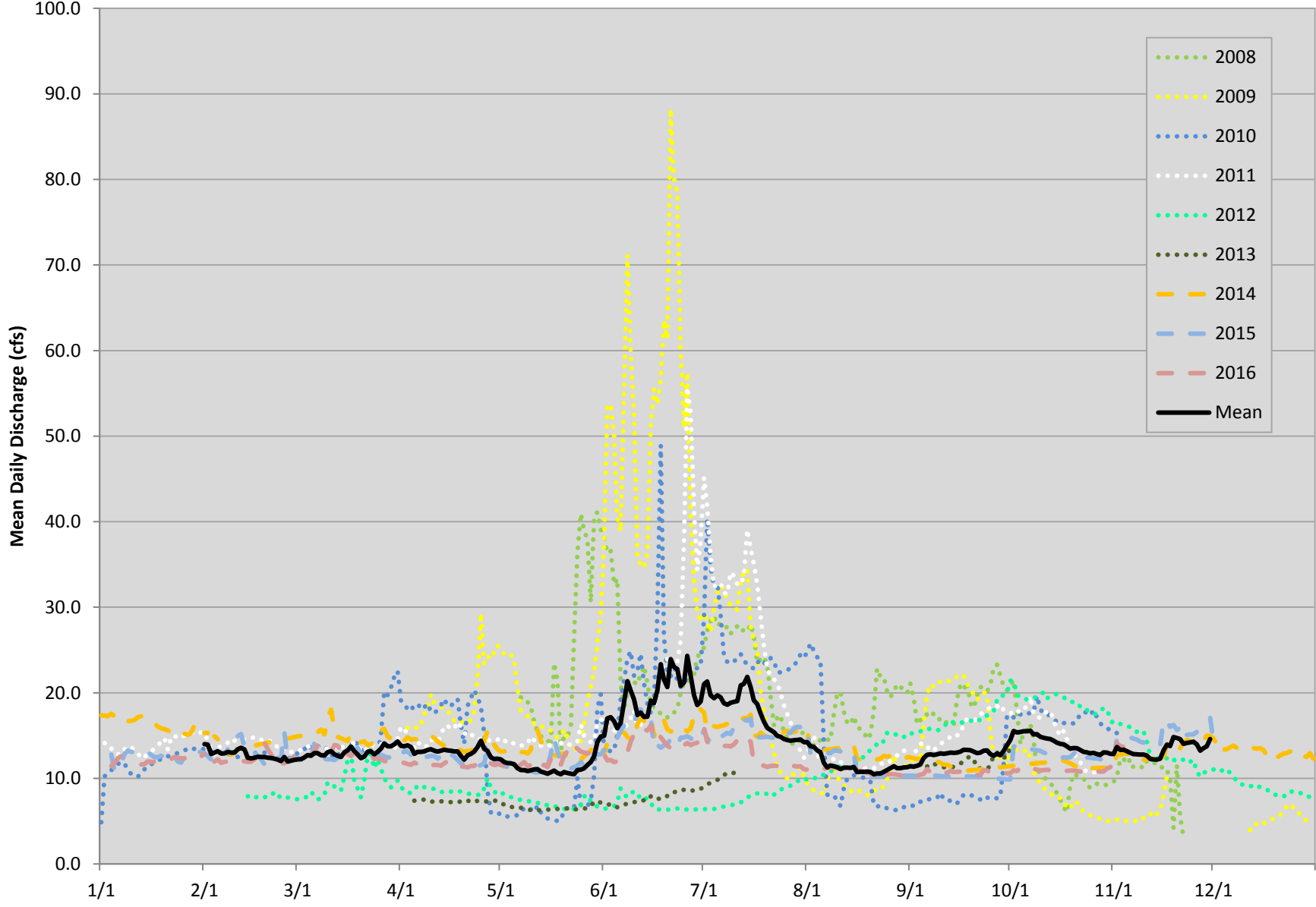
Upper Little Springs Creek Flows 2008-2016
