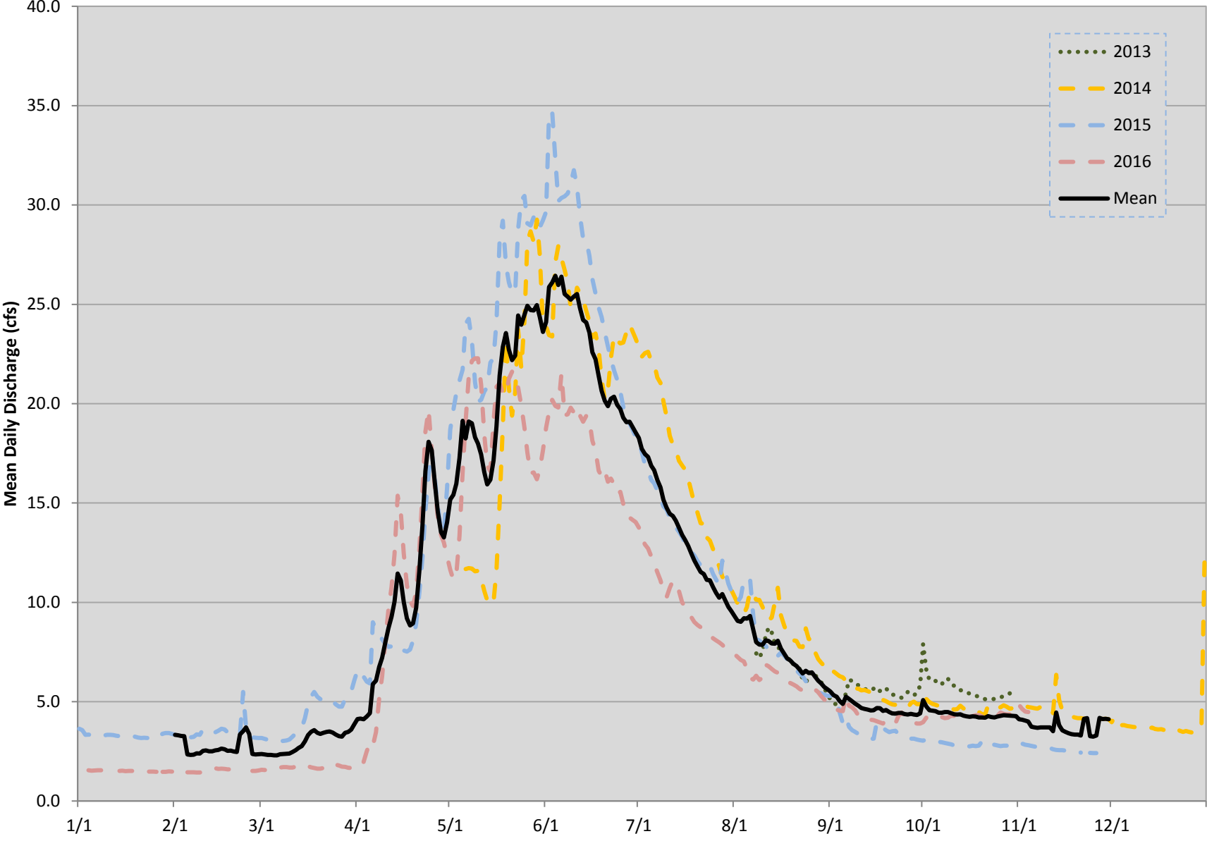
Upper Bohannon Creek Flows 2013-2016
