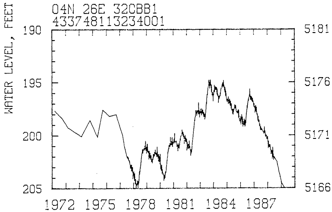
FIGURE 9. Hydrographs of wells 03N26E22ABA1 and 04N26E32CBB1.
