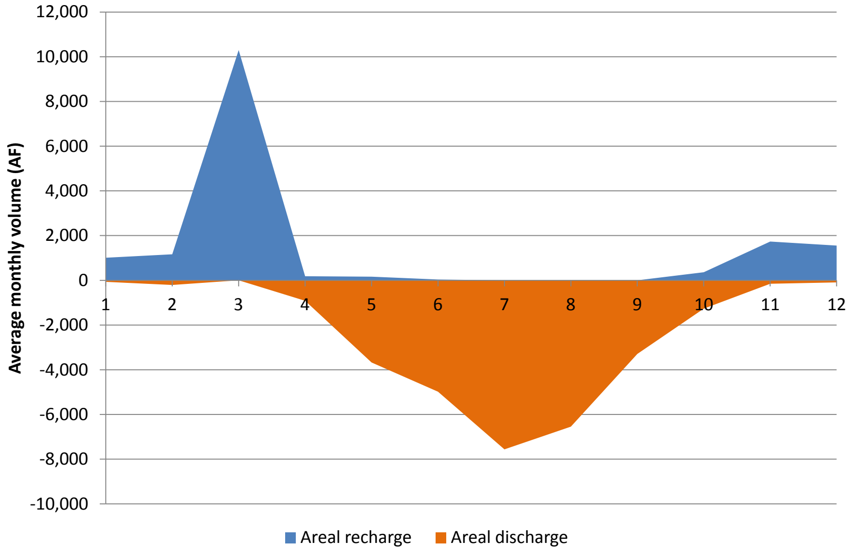
Average monthly non-irrigated areal recharge and discharge (1995-2010)
