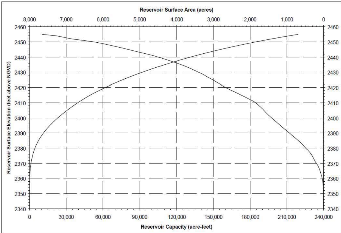
Figure B.2-4 C.J. Strike Reservoir area and capacity curves.
