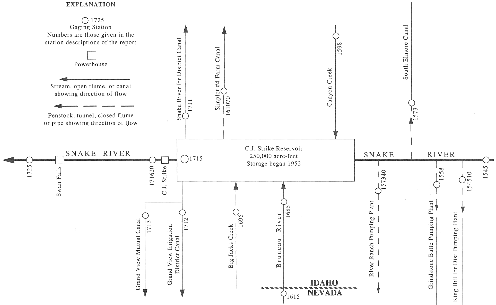
Figure 13. Gaging stations in the Snake River basin between King Hill and Murphy and the Bruneau River basin.
