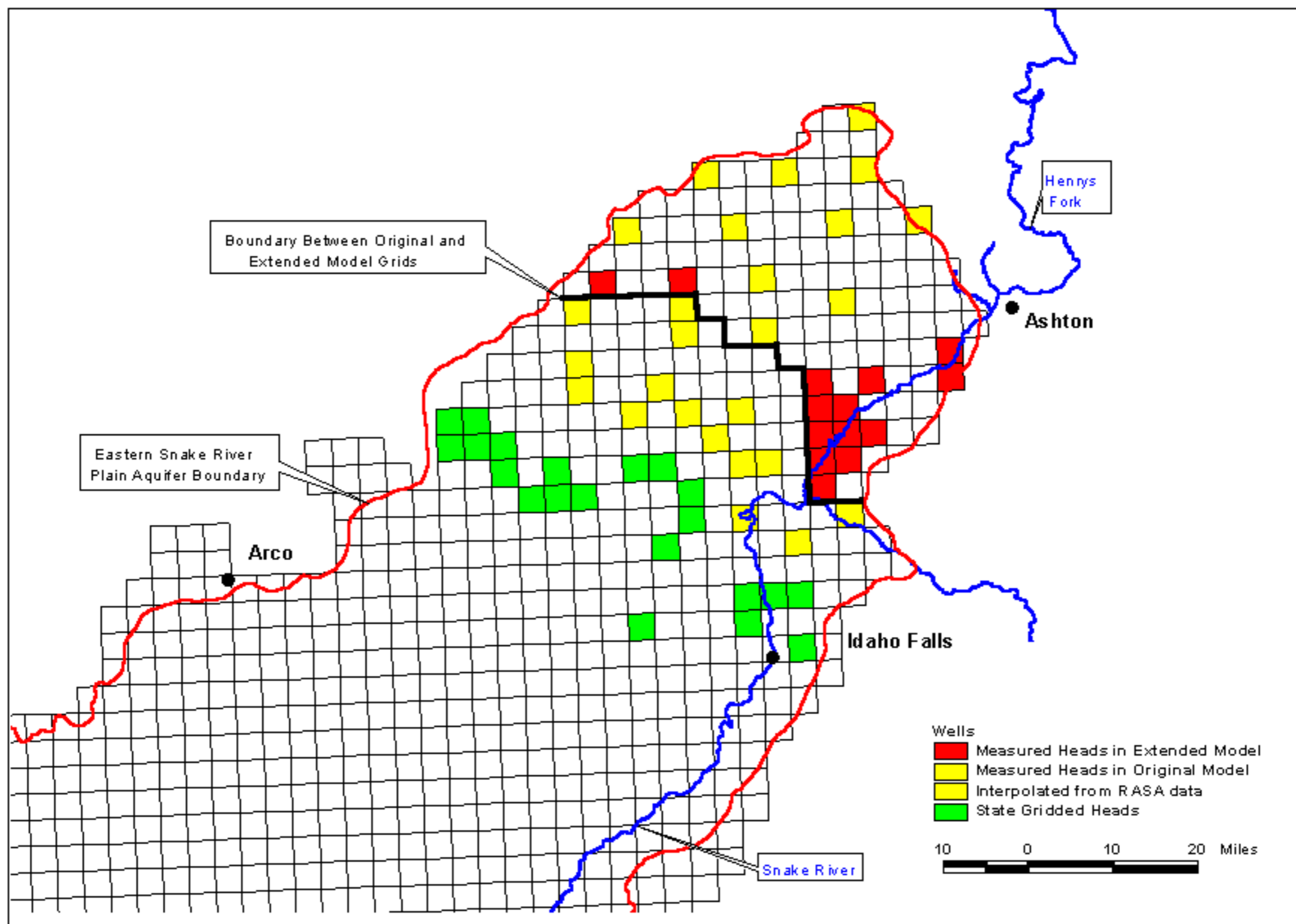
Figure 5. Location of Model Cells Containing Water Level Calibration Targets.
