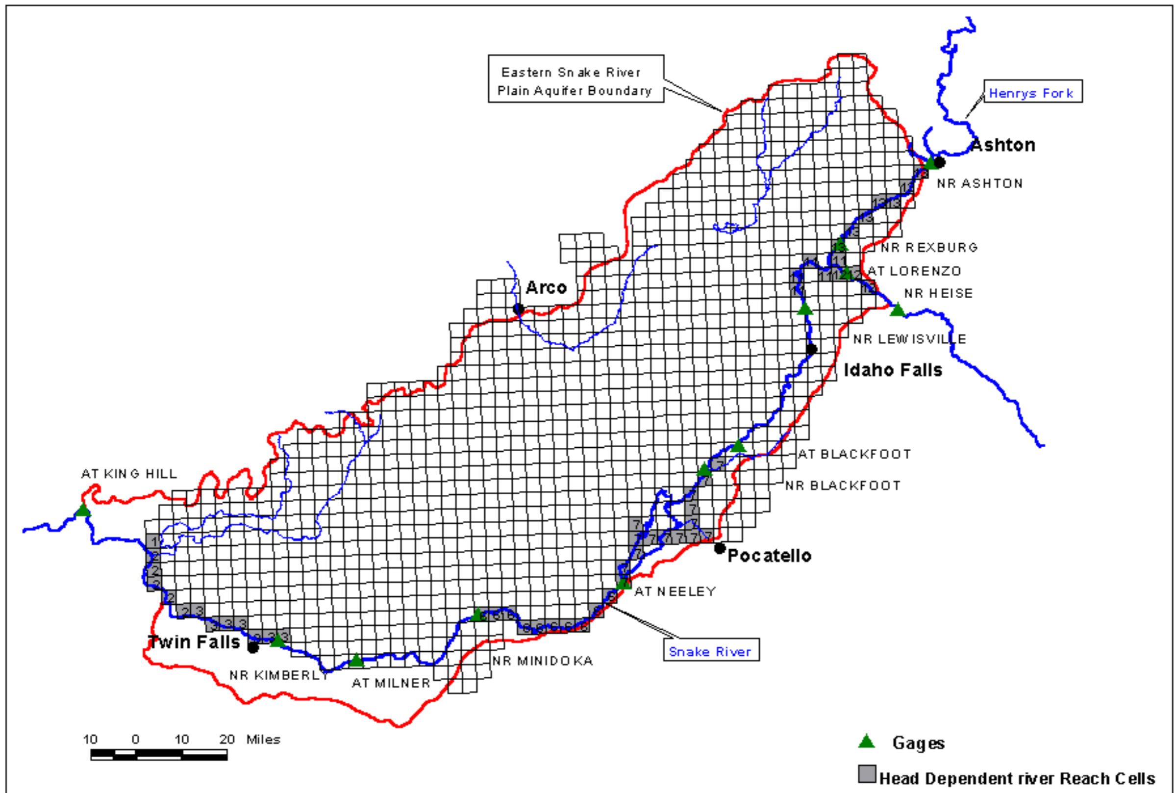
Figure 6. Location of River Reaches Used in Model Calibration.
