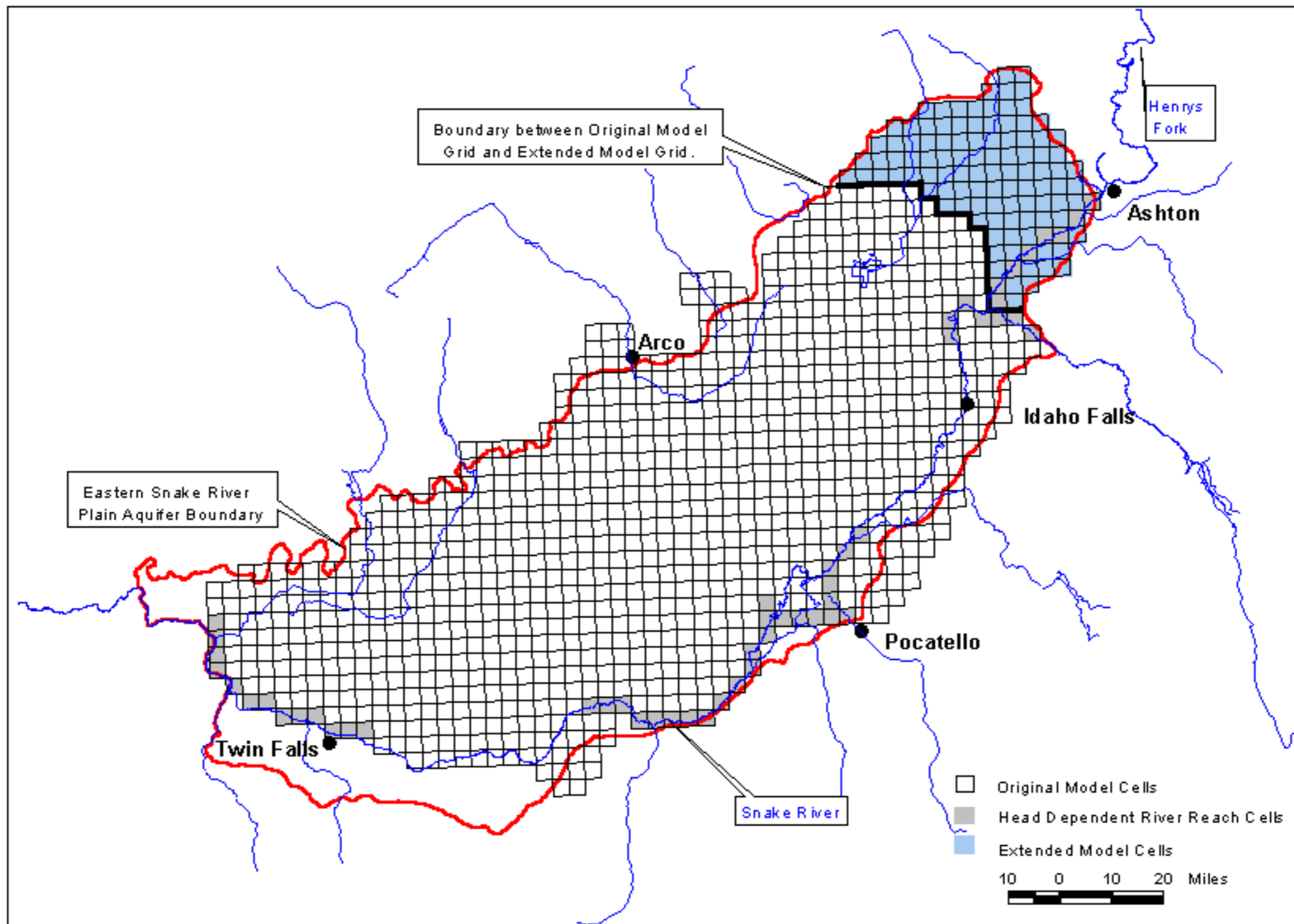
Figure 2. IDWR/UI Ground Water Flow Model Grid and RASA Boundary.
