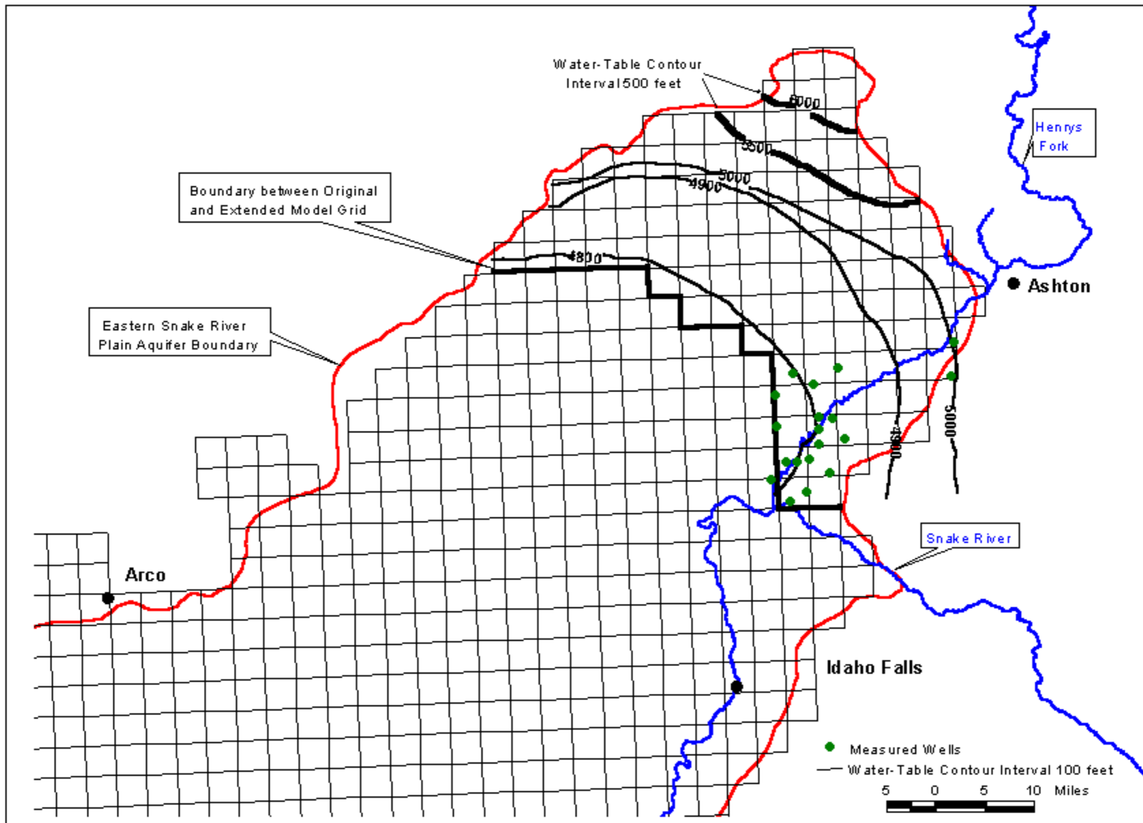
Figure 4. Water Level Contours From Measured Wells in the Expanded Model Area.
