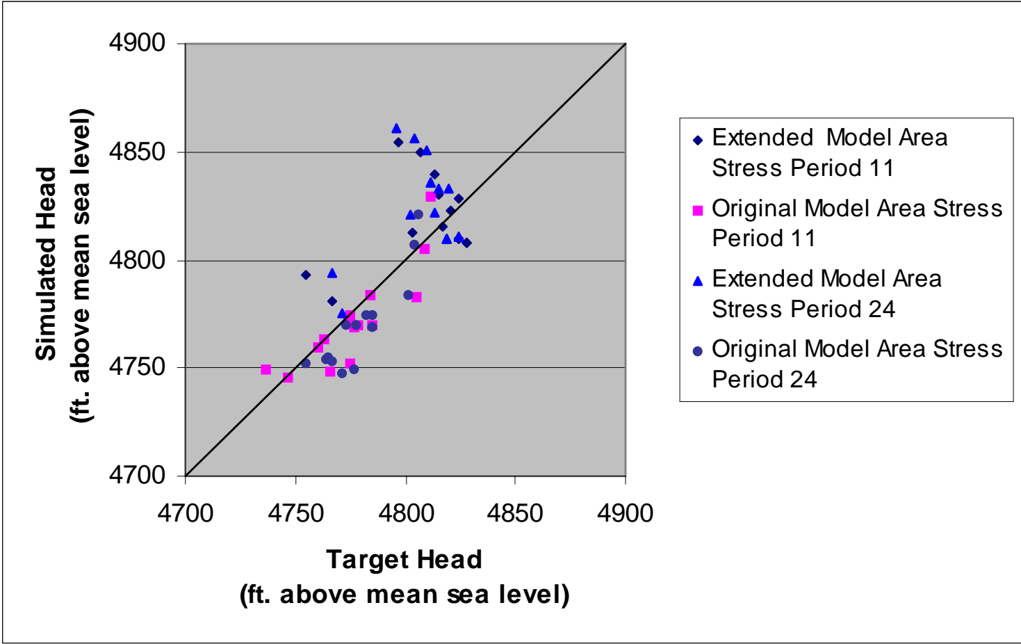
Figure 7. Scatter Plot of Simulated Heads vs. Target Heads for Stress Periods 11 and 24.
