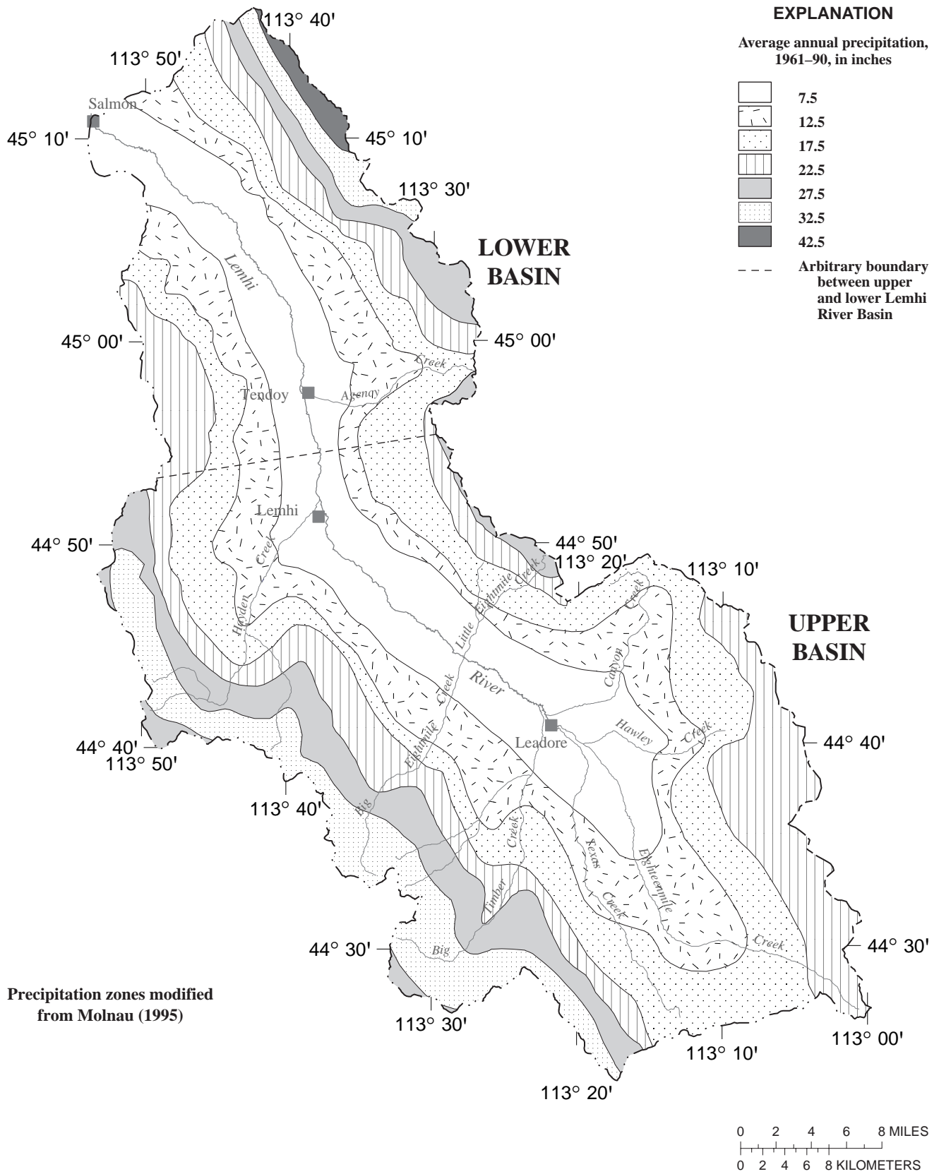
Figure 3. Average annual precipitation in the Lemhi River Basin, east-central Idaho, 1961-90.
