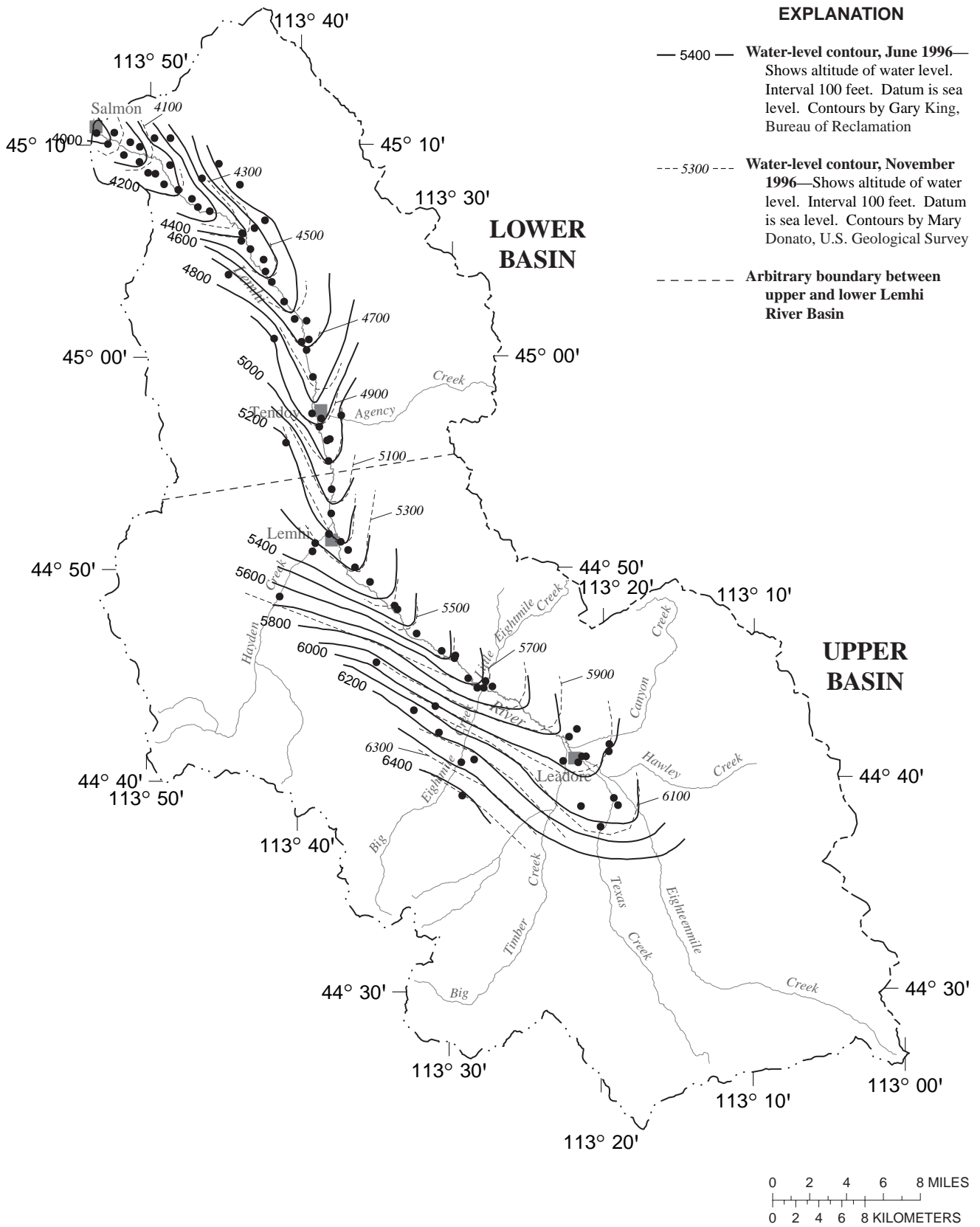
Figure 8. Ground-water level contours in the Lemhi River Basin, east-central Idaho, June and November 1996.
