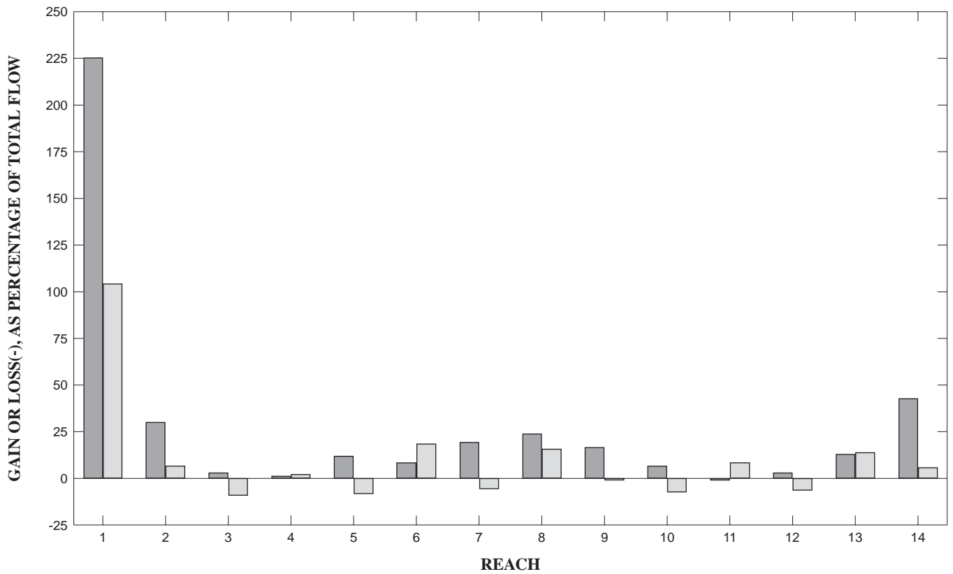
Figure 7. Gains and losses, in cubic feet per second per mile and as a percentage of total flow in the Lemhi River, east-central Idaho, August and October 1997.
