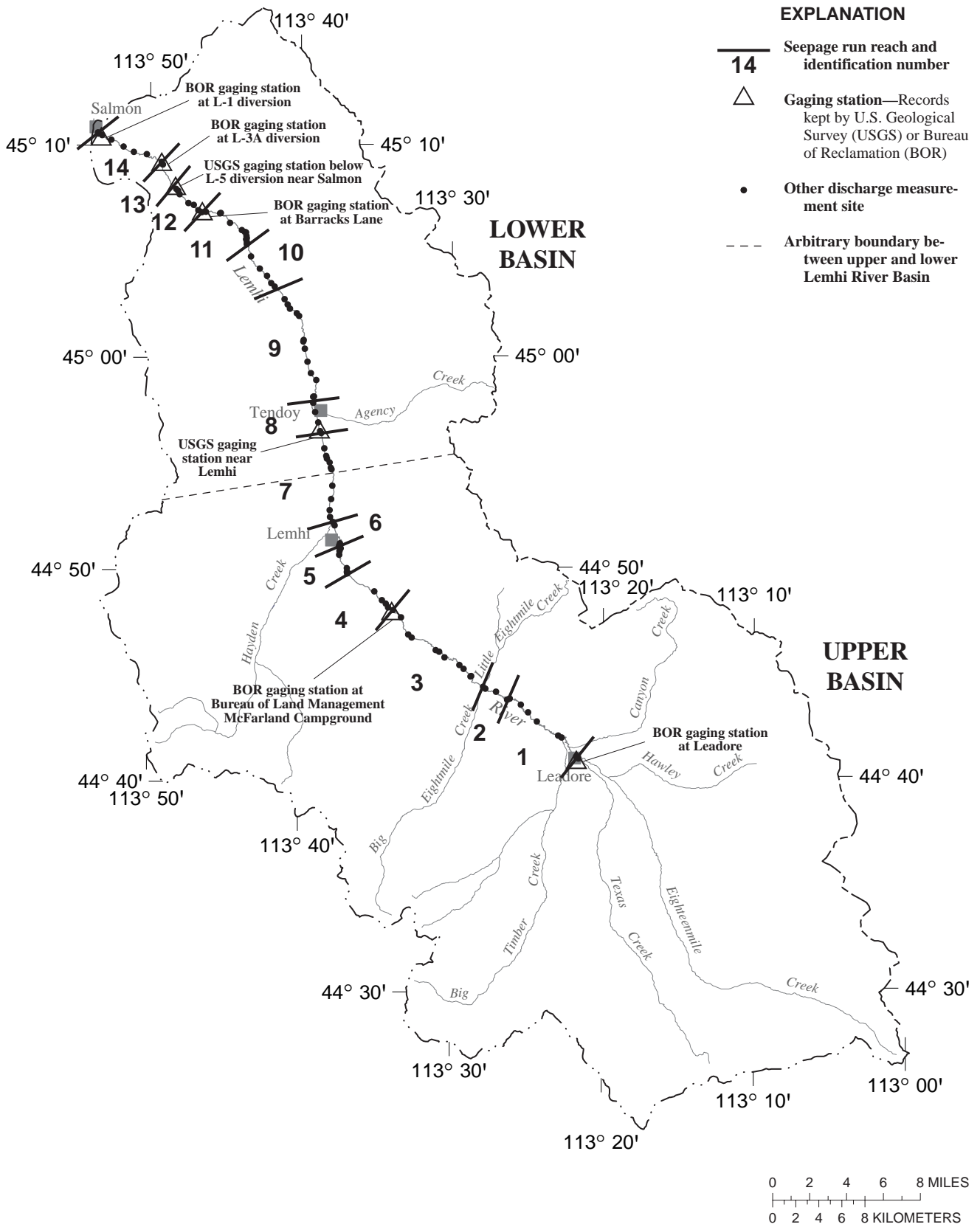
Figure 4. Seepage run reaches, gaging stations, and discharge measurement sites in the Lemhi River Basin, east-central Idaho, August and October 1997. (Data listed in appendices 1 and 2)
