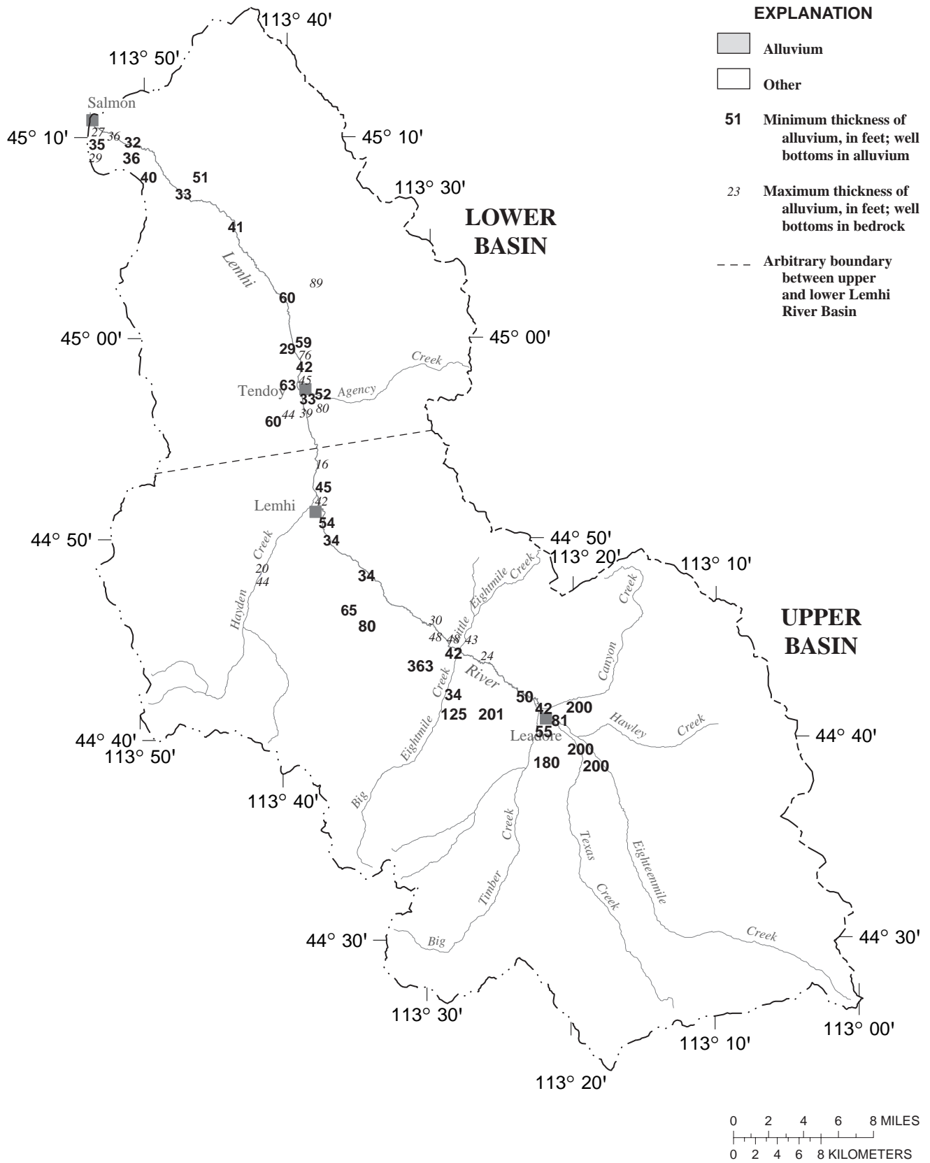
Figure 2. Estimated thickness of alluvium in the Lemhi River Basin, east-central Idaho.
