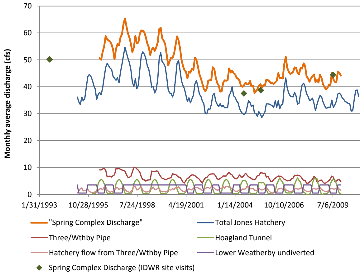
Figure 2. Estimated spring discharge at Three Springs, Weatherby Springs, and Hoagland Tunnel.
