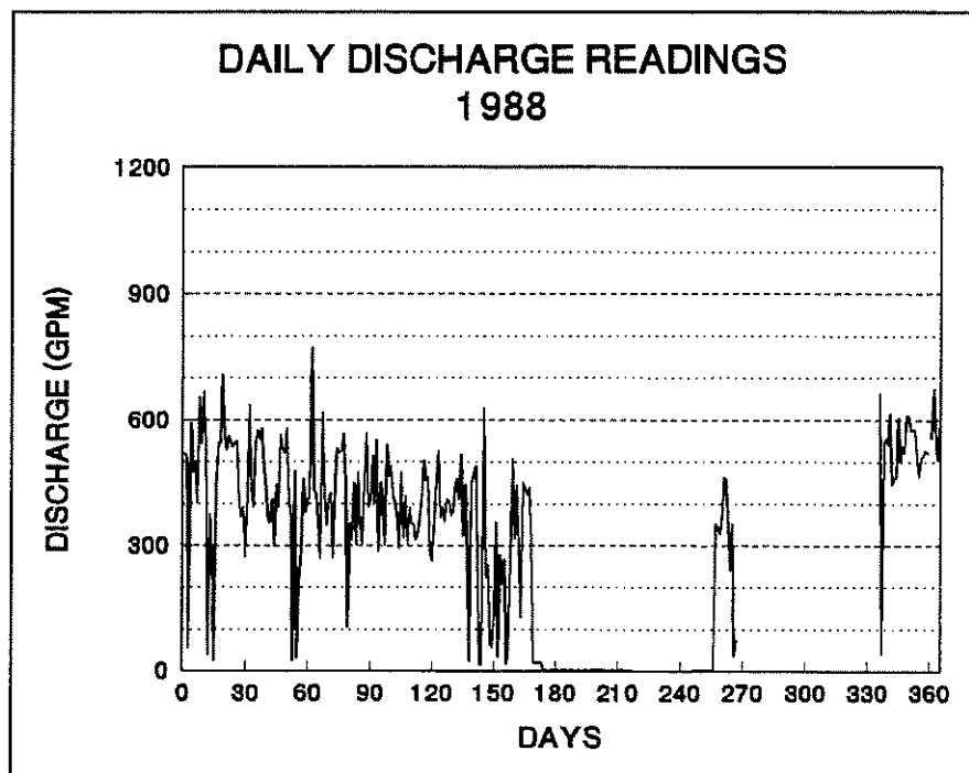
Figure 12. Daily discharge readings for the Capitol Mall geothermal system, 1988.
